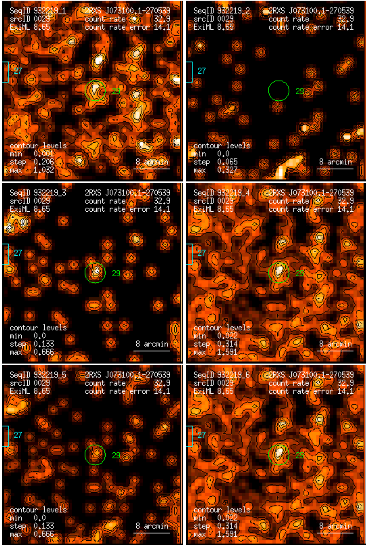
Figure 29: RASS 932219: detection 0029: band rate images, Gaussian filter: (1) PSPC channels 11 – 41, (2) 52 – 90, (3) 91 – 201, (4) 11 – 235, (5) 52 – 201, (6) 11 – 201. Broad band rates in counts/ks. Band rate contour levels in counts/ks/arcmin 2 .
