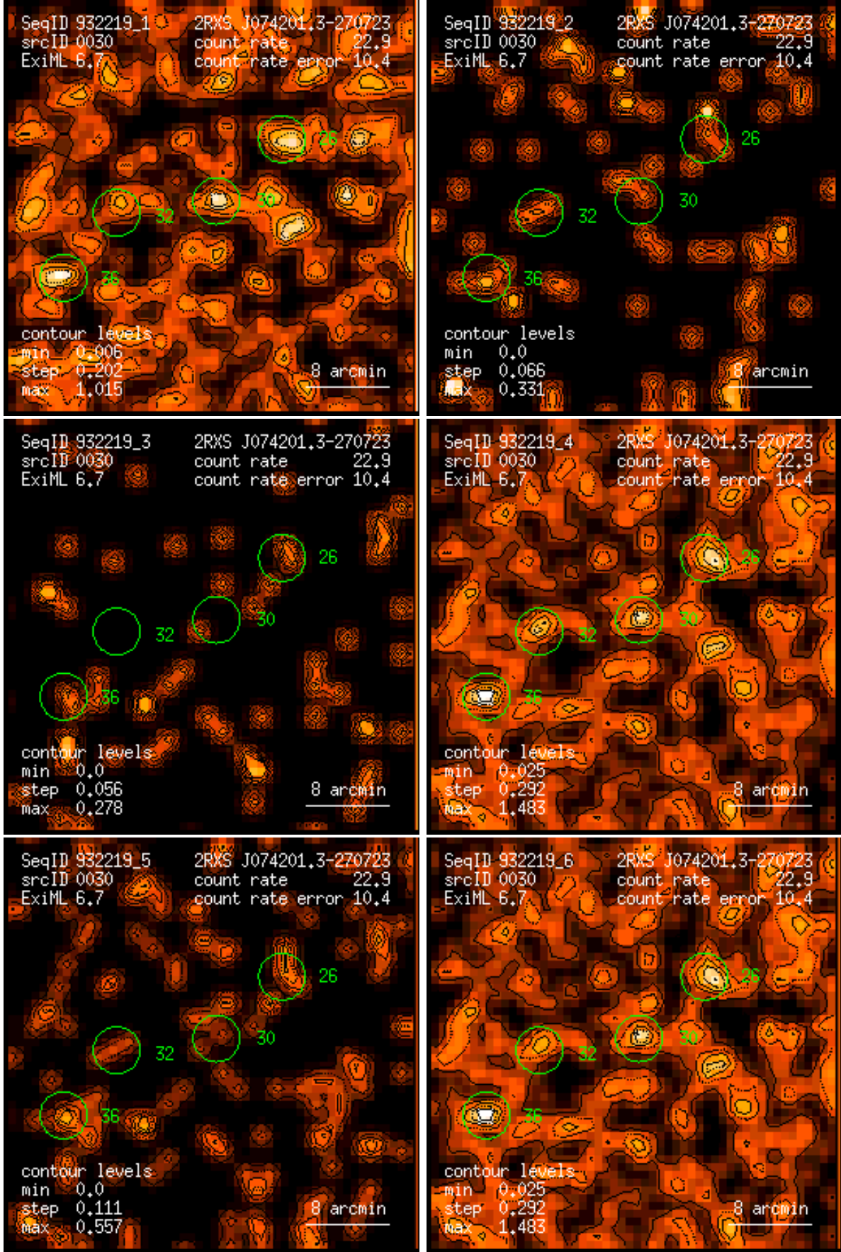
Figure 30: RASS 932219: detection 0030: band rate images, Gaussian filter: (1) PSPC channels 11 – 41, (2) 52 – 90, (3) 91 – 201, (4) 11 – 235, (5) 52 – 201, (6) 11 – 201. Broad band rates in counts/ks. Band rate contour levels in counts/ks/arcmin 2 .
