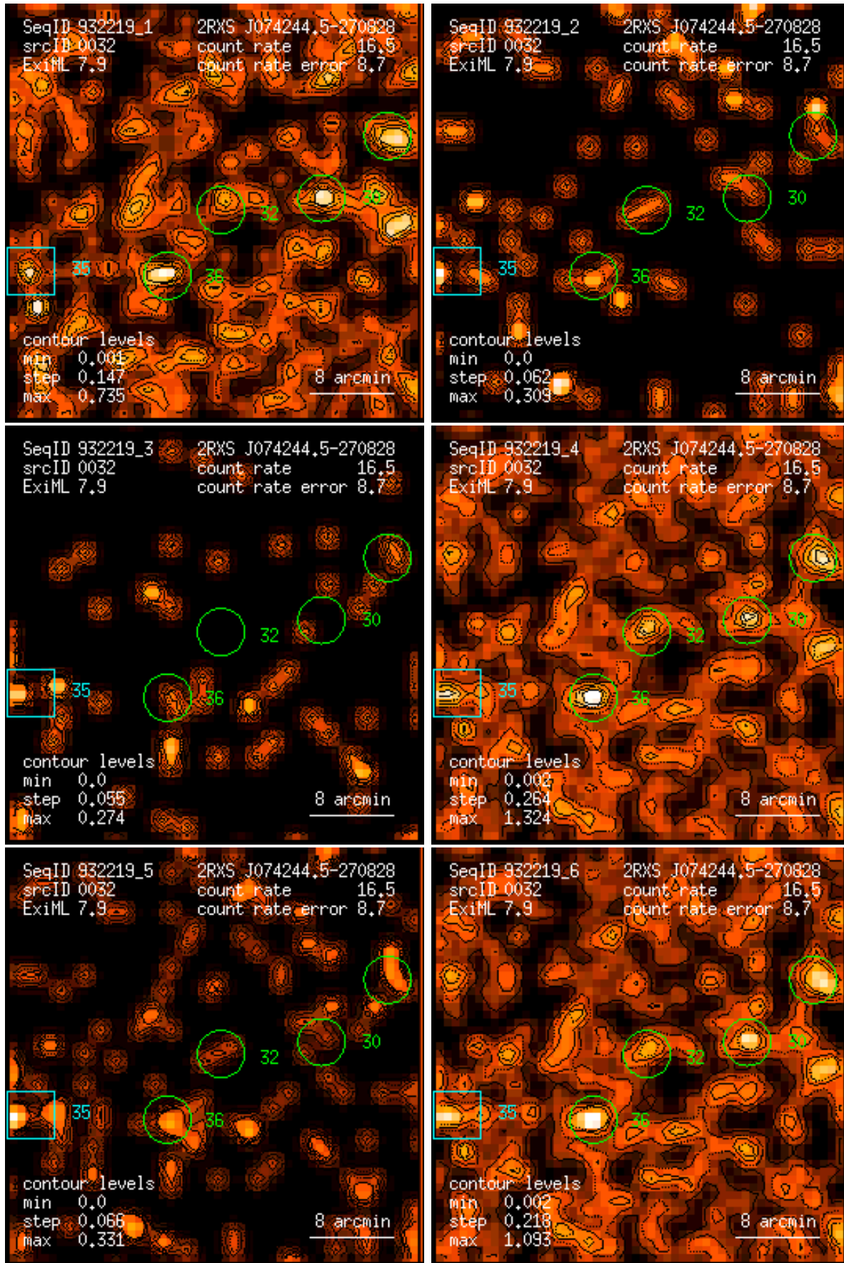
Figure 32: RASS 932219: detection 0032: band rate images, Gaussian filter: (1) PSPC channels 11 – 41, (2) 52 – 90, (3) 91 – 201, (4) 11 – 235, (5) 52 – 201, (6) 11 – 201. Broad band rates in counts/ks. Band rate contour levels in counts/ks/arcmin 2 .
