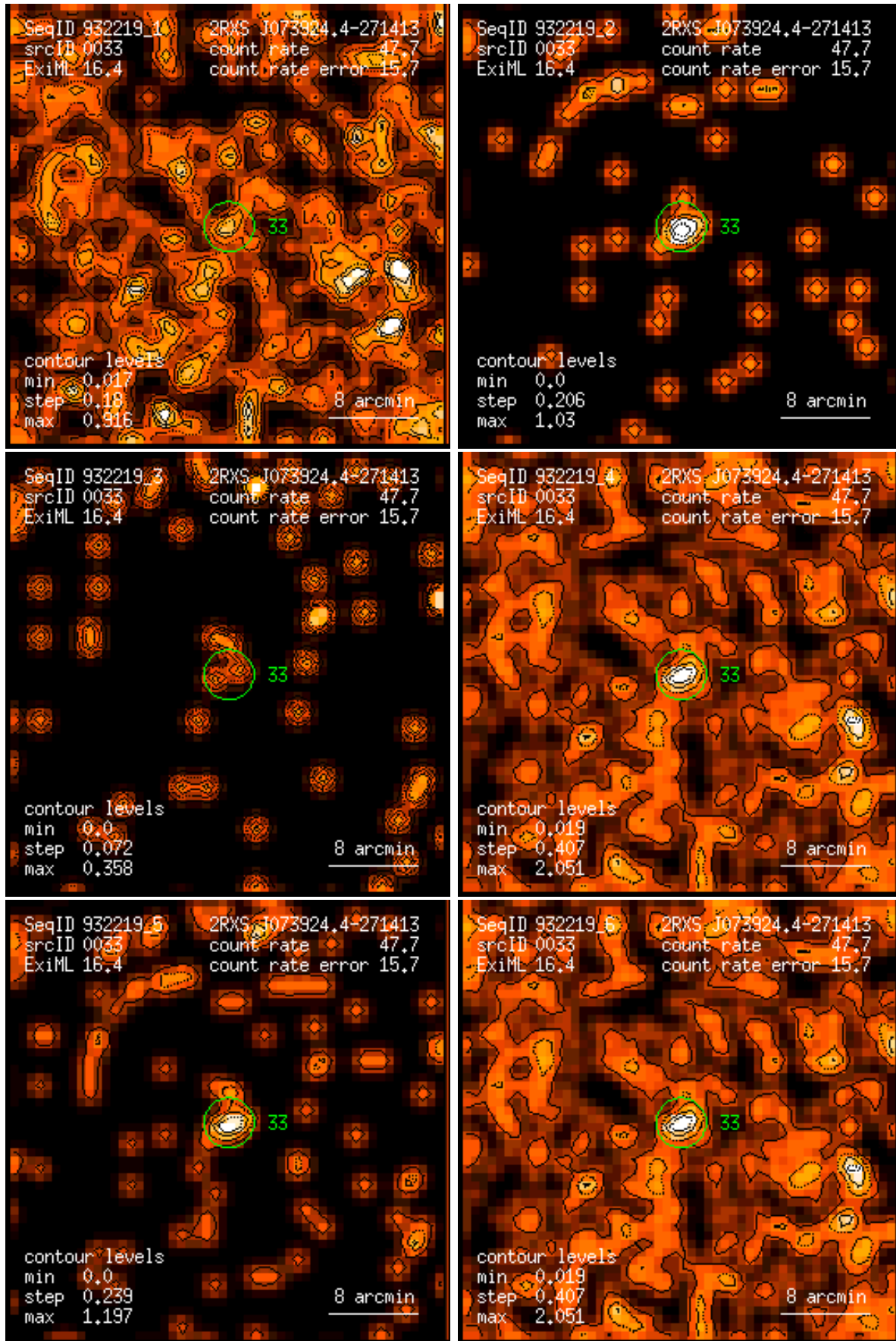
Figure 33: RASS 932219: detection 0033: band rate images, Gaussian filter: (1) PSPC channels 11 – 41, (2) 52 – 90, (3) 91 – 201, (4) 11 – 235, (5) 52 – 201, (6) 11 – 201. Broad band rates in counts/ks. Band rate contour levels in counts/ks/arcmin 2 .
