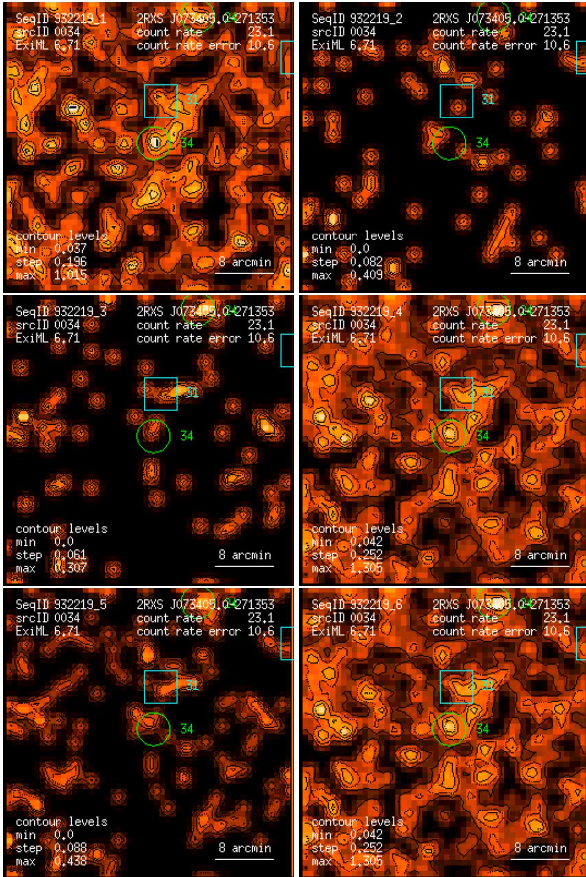
Figure 34: RASS 932219: detection 0034: band rate images, Gaussian filter: (1) PSPC channels 11 – 41, (2) 52 – 90, (3) 91 – 201, (4) 11 – 235, (5) 52 – 201, (6) 11 – 201. Broad band rates in counts/ks. Band rate contour levels in counts/ks/arcmin 2 .
