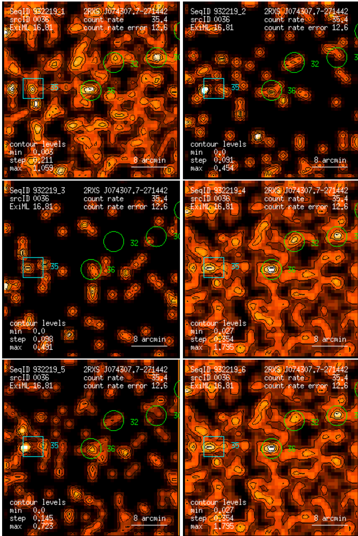
Figure 36: RASS 932219: detection 0036: band rate images, Gaussian filter: (1) PSPC channels 11 – 41, (2) 52 – 90, (3) 91 – 201, (4) 11 – 235, (5) 52 – 201, (6) 11 – 201. Broad band rates in counts/ks. Band rate contour levels in counts/ks/arcmin 2 .
