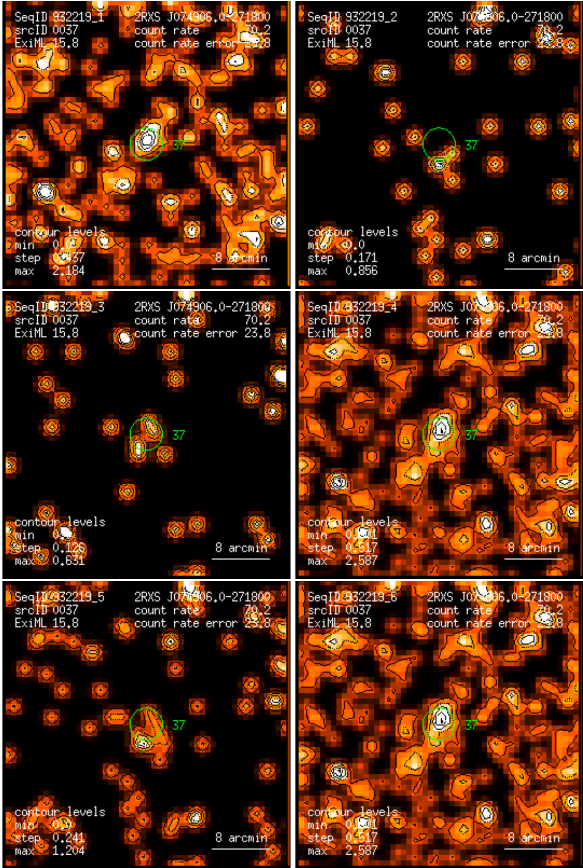
Figure 37: RASS 932219: detection 0037: band rate images, Gaussian filter: (1) PSPC channels 11 – 41, (2) 52 – 90, (3) 91 – 201, (4) 11 – 235, (5) 52 – 201, (6) 11 – 201. Broad band rates in counts/ks. Band rate contour levels in counts/ks/arcmin 2 .
