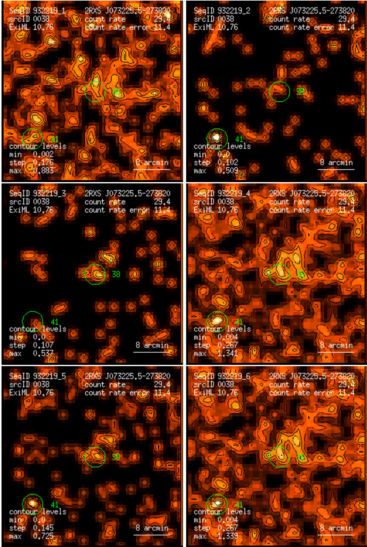
Figure 38: RASS 932219: detection 0038: band rate images, Gaussian filter: (1) PSPC channels 11 – 41, (2) 52 – 90, (3) 91 – 201, (4) 11 – 235, (5) 52 – 201, (6) 11 – 201. Broad band rates in counts/ks. Band rate contour levels in counts/ks/arcmin 2 .
