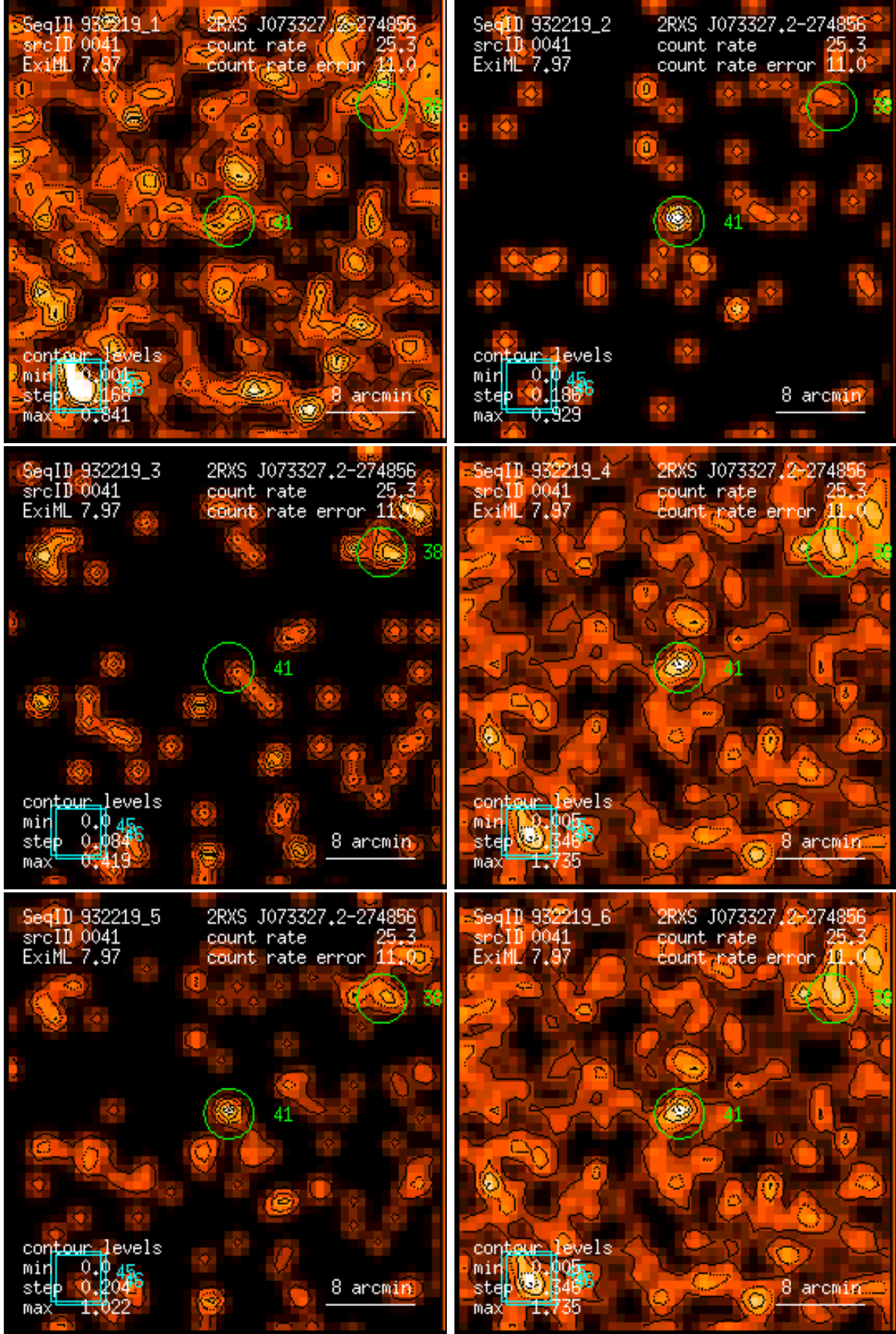
Figure 41: RASS 932219: detection 0041: band rate images, Gaussian filter: (1) PSPC channels 11 – 41, (2) 52 – 90, (3) 91 – 201, (4) 11 – 235, (5) 52 – 201, (6) 11 – 201. Broad band rates in counts/ks. Band rate contour levels in counts/ks/arcmin 2 .
