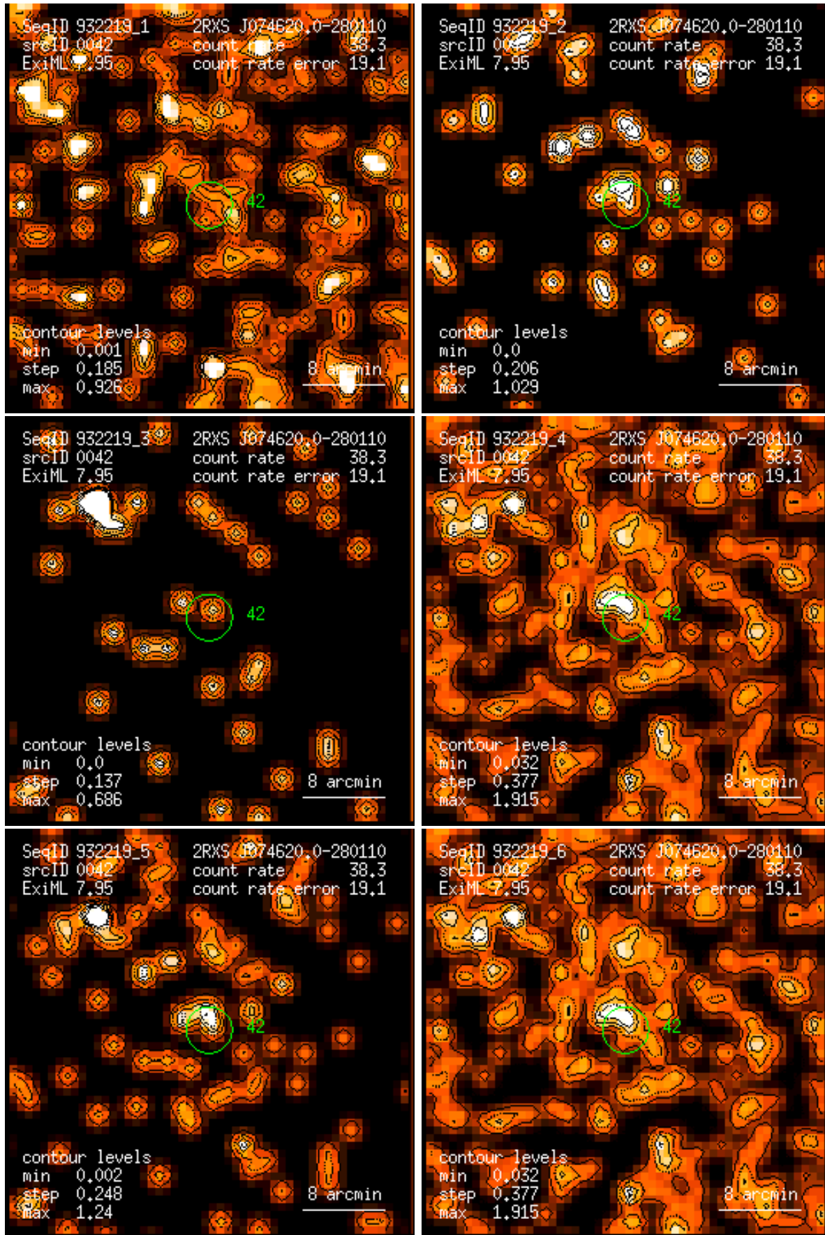
Figure 42: RASS 932219: detection 0042: band rate images, Gaussian filter: (1) PSPC channels 11 – 41, (2) 52 – 90, (3) 91 – 201, (4) 11 – 235, (5) 52 – 201, (6) 11 – 201. Broad band rates in counts/ks. Band rate contour levels in counts/ks/arcmin 2 .
