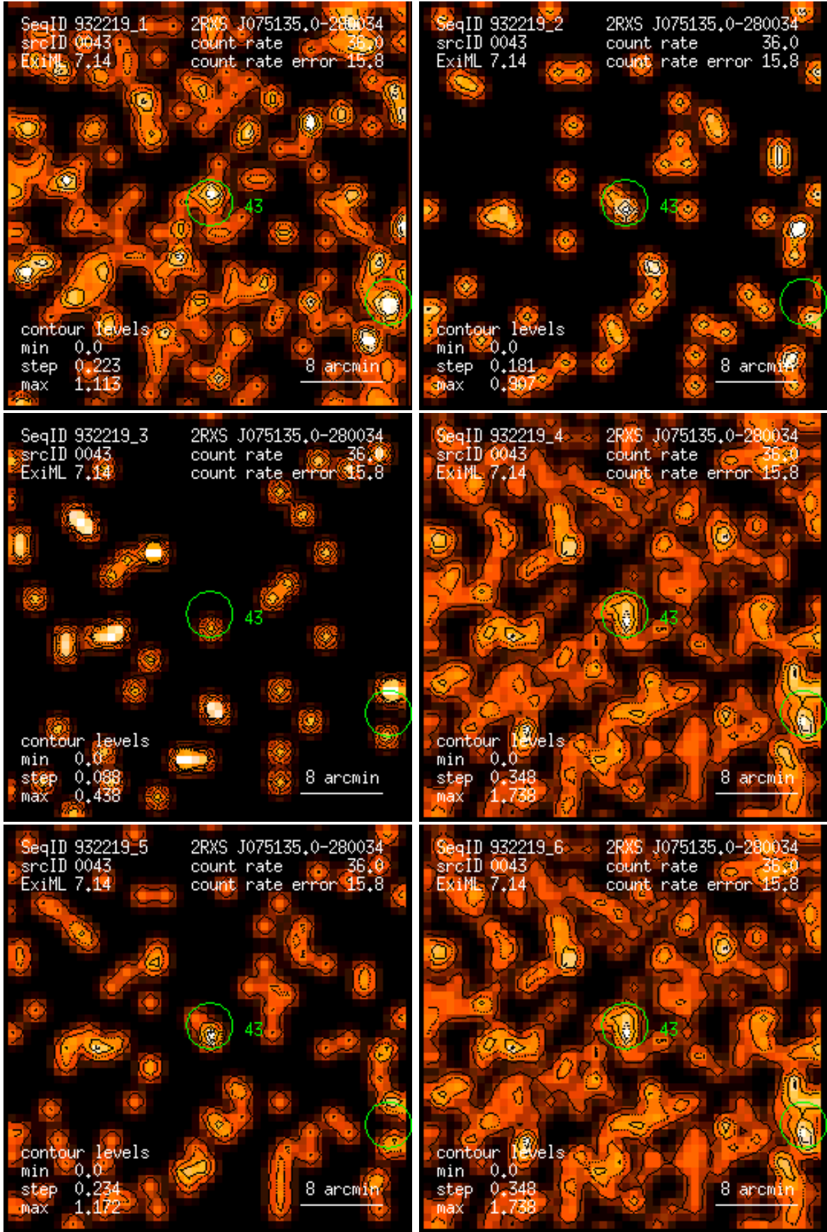
Figure 43: RASS 932219: detection 0043: band rate images, Gaussian filter: (1) PSPC channels 11 – 41, (2) 52 – 90, (3) 91 – 201, (4) 11 – 235, (5) 52 – 201, (6) 11 – 201. Broad band rates in counts/ks. Band rate contour levels in counts/ks/arcmin 2 .
