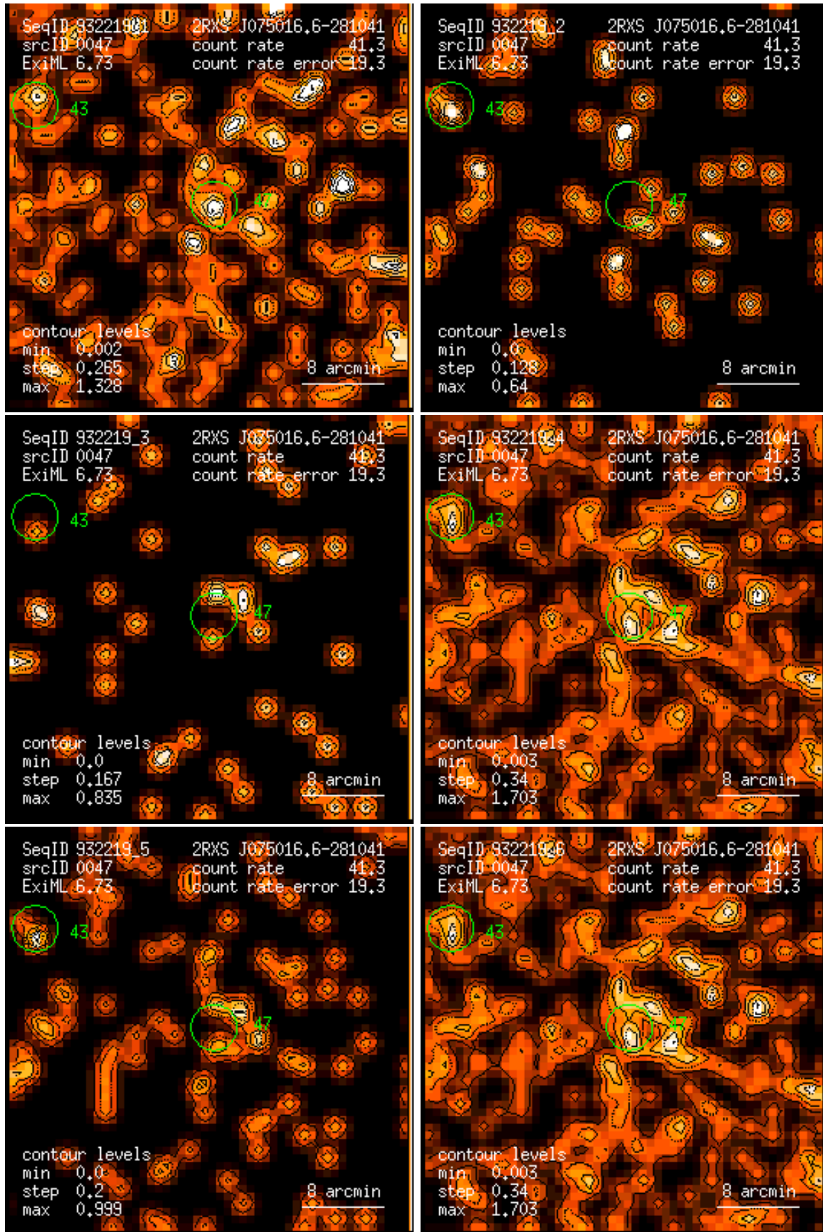
Figure 47: RASS 932219: detection 0047: band rate images, Gaussian filter: (1) PSPC channels 11 – 41, (2) 52 – 90, (3) 91 – 201, (4) 11 – 235, (5) 52 – 201, (6) 11 – 201. Broad band rates in counts/ks. Band rate contour levels in counts/ks/arcmin 2 .
