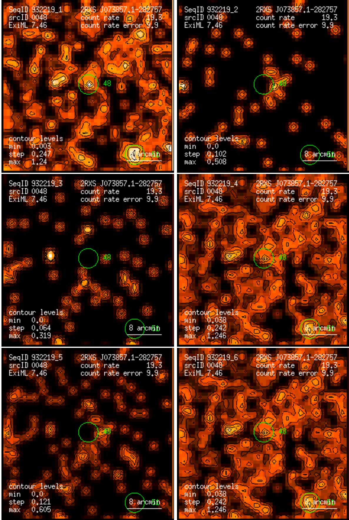
Figure 48: RASS 932219: detection 0048: band rate images, Gaussian filter: (1) PSPC channels 11 – 41, (2) 52 – 90, (3) 91 – 201, (4) 11 – 235, (5) 52 – 201, (6) 11 – 201. Broad band rates in counts/ks. Band rate contour levels in counts/ks/arcmin 2 .
