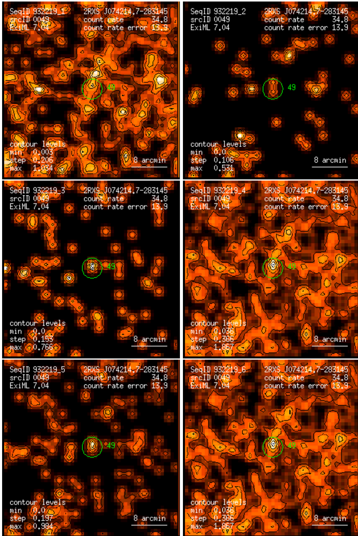
Figure 49: RASS 932219: detection 0049: band rate images, Gaussian filter: (1) PSPC channels 11 – 41, (2) 52 – 90, (3) 91 – 201, (4) 11 – 235, (5) 52 – 201, (6) 11 – 201. Broad band rates in counts/ks. Band rate contour levels in counts/ks/arcmin 2 .
