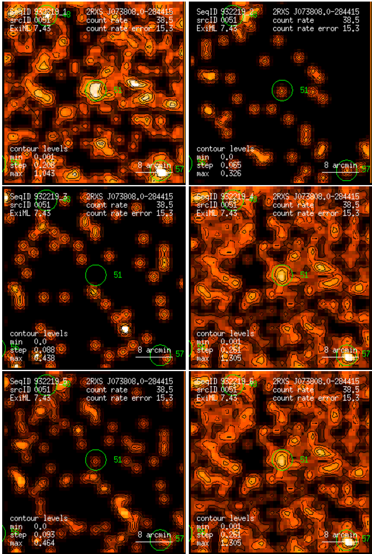
Figure 51: RASS 932219: detection 0051: band rate images, Gaussian filter: (1) PSPC channels 11 – 41, (2) 52 – 90, (3) 91 – 201, (4) 11 – 235, (5) 52 – 201, (6) 11 – 201. Broad band rates in counts/ks. Band rate contour levels in counts/ks/arcmin 2 .
