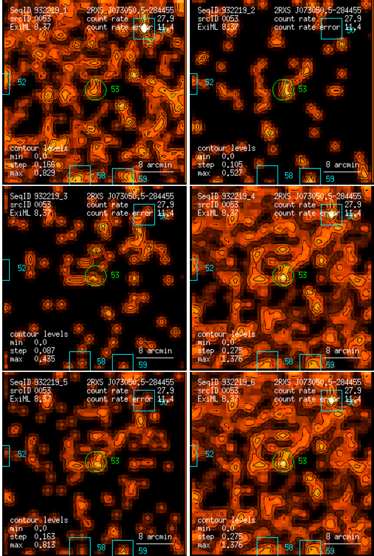
Figure 53: RASS 932219: detection 0053: band rate images, Gaussian filter: (1) PSPC channels 11 – 41, (2) 52 – 90, (3) 91 – 201, (4) 11 – 235, (5) 52 – 201, (6) 11 – 201. Broad band rates in counts/ks. Band rate contour levels in counts/ks/arcmin 2 .
