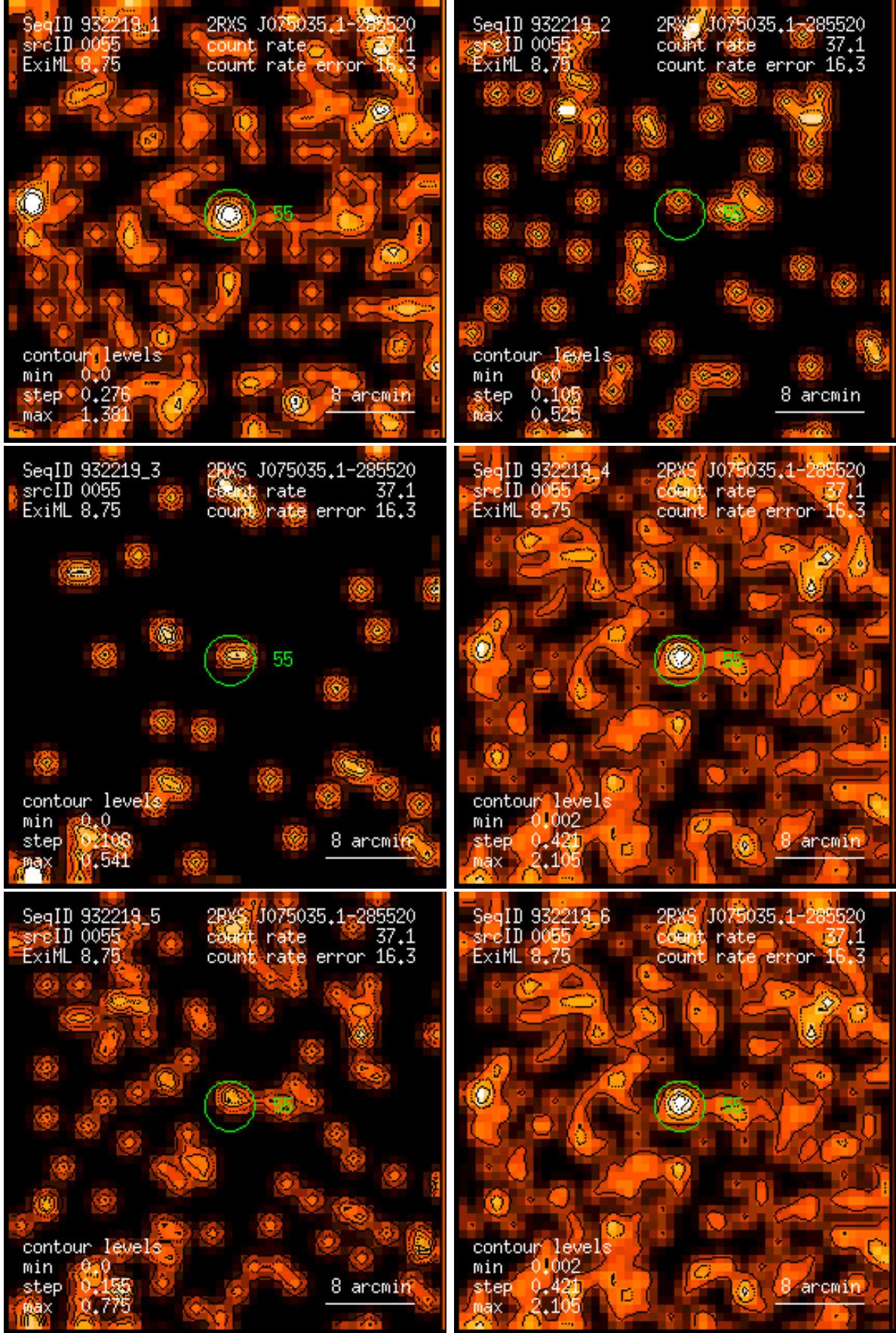
Figure 55: RASS 932219: detection 0055: band rate images, Gaussian filter: (1) PSPC channels 11 – 41, (2) 52 – 90, (3) 91 – 201, (4) 11 – 235, (5) 52 – 201, (6) 11 – 201. Broad band rates in counts/ks. Band rate contour levels in counts/ks/arcmin 2 .
