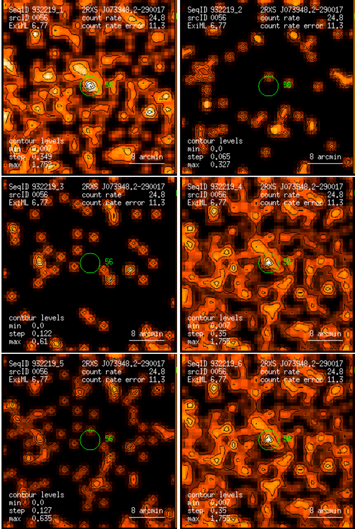
Figure 56: RASS 932219: detection 0056: band rate images, Gaussian filter: (1) PSPC channels 11 – 41, (2) 52 – 90, (3) 91 – 201, (4) 11 – 235, (5) 52 – 201, (6) 11 – 201. Broad band rates in counts/ks. Band rate contour levels in counts/ks/arcmin 2 .
