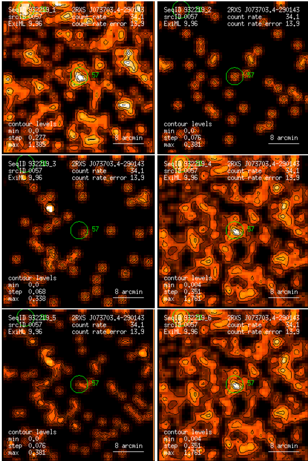
Figure 57: RASS 932219: detection 0057: band rate images, Gaussian filter: (1) PSPC channels 11 – 41, (2) 52 – 90, (3) 91 – 201, (4) 11 – 235, (5) 52 – 201, (6) 11 – 201. Broad band rates in counts/ks. Band rate contour levels in counts/ks/arcmin 2 .
