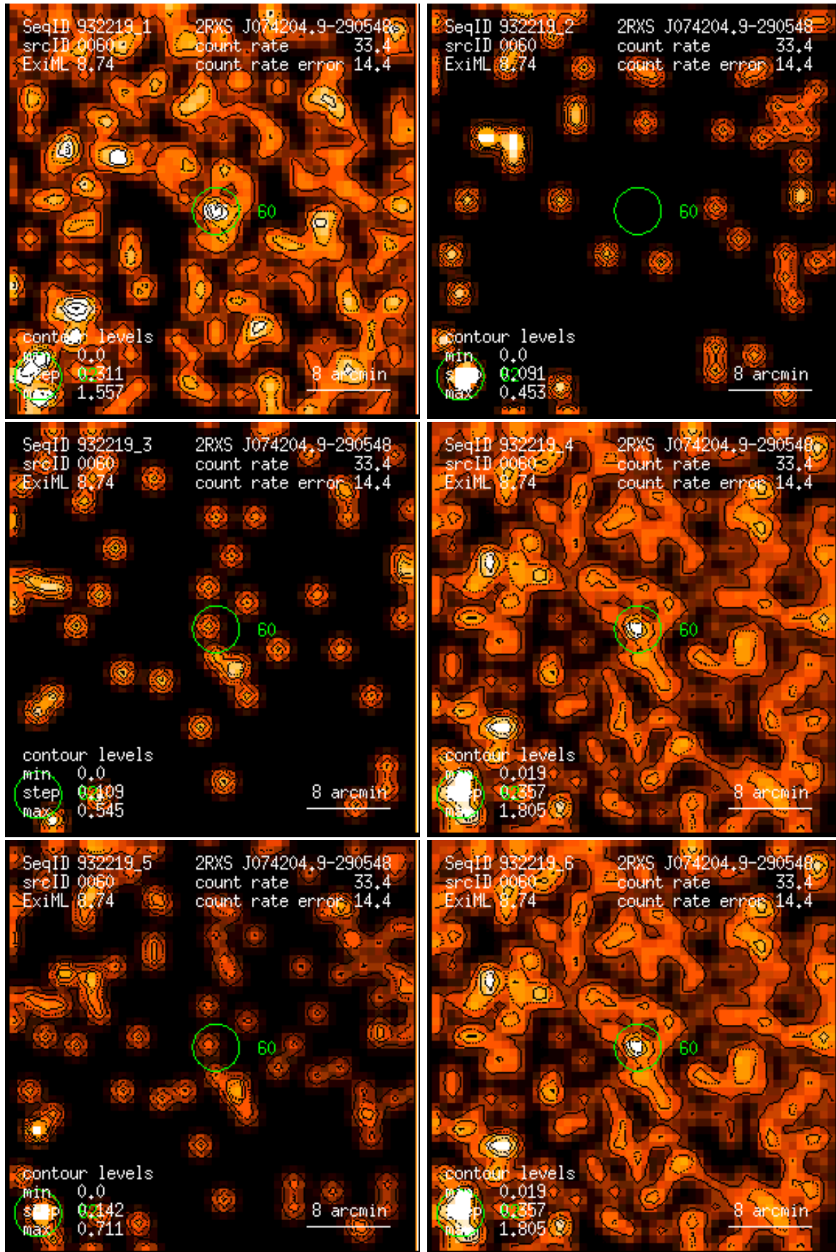
Figure 60: RASS 932219: detection 0060: band rate images, Gaussian filter: (1) PSPC channels 11 – 41, (2) 52 – 90, (3) 91 – 201, (4) 11 – 235, (5) 52 – 201, (6) 11 – 201. Broad band rates in counts/ks. Band rate contour levels in counts/ks/arcmin 2 .
