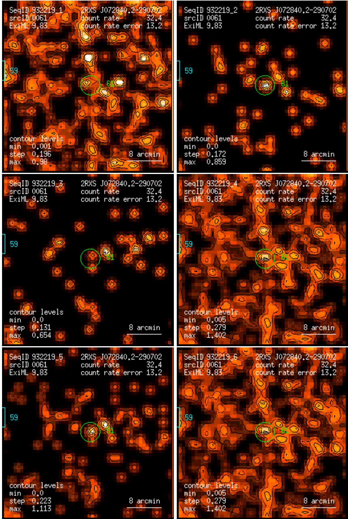
Figure 61: RASS 932219: detection 0061: band rate images, Gaussian filter: (1) PSPC channels 11 – 41, (2) 52 – 90, (3) 91 – 201, (4) 11 – 235, (5) 52 – 201, (6) 11 – 201. Broad band rates in counts/ks. Band rate contour levels in counts/ks/arcmin 2 .
