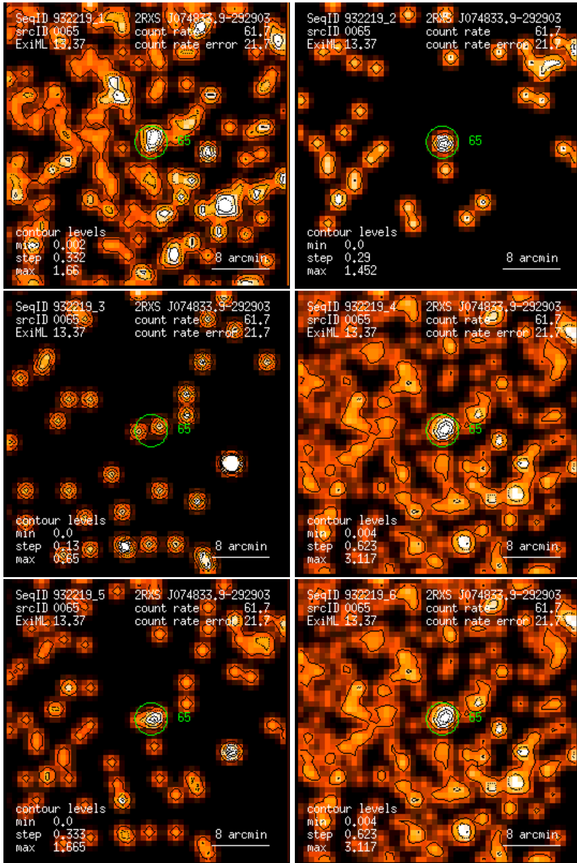
Figure 65: RASS 932219: detection 0065: band rate images, Gaussian filter: (1) PSPC channels 11 – 41, (2) 52 – 90, (3) 91 – 201, (4) 11 – 235, (5) 52 – 201, (6) 11 – 201. Broad band rates in counts/ks. Band rate contour levels in counts/ks/arcmin 2 .
