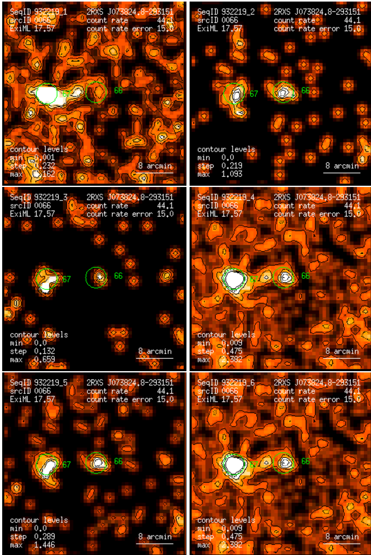
Figure 66: RASS 932219: detection 0066: band rate images, Gaussian filter: (1) PSPC channels 11 – 41, (2) 52 – 90, (3) 91 – 201, (4) 11 – 235, (5) 52 – 201, (6) 11 – 201. Broad band rates in counts/ks. Band rate contour levels in counts/ks/arcmin 2 .
