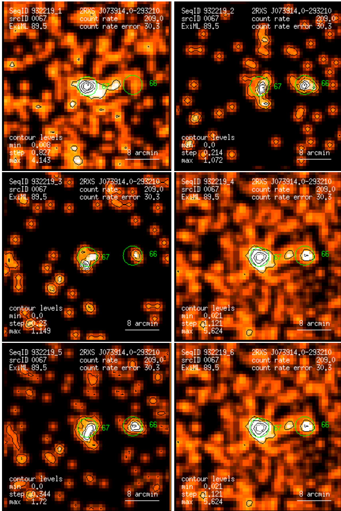
Figure 67: RASS 932219: detection 0067: band rate images, Gaussian filter: (1) PSPC channels 11 – 41, (2) 52 – 90, (3) 91 – 201, (4) 11 – 235, (5) 52 – 201, (6) 11 – 201. Broad band rates in counts/ks. Band rate contour levels in counts/ks/arcmin 2 .
