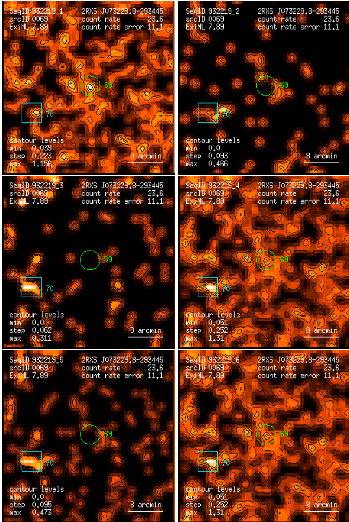
Figure 69: RASS 932219: detection 0069: band rate images, Gaussian filter: (1) PSPC channels 11 – 41, (2) 52 – 90, (3) 91 – 201, (4) 11 – 235, (5) 52 – 201, (6) 11 – 201. Broad band rates in counts/ks. Band rate contour levels in counts/ks/arcmin 2 .
