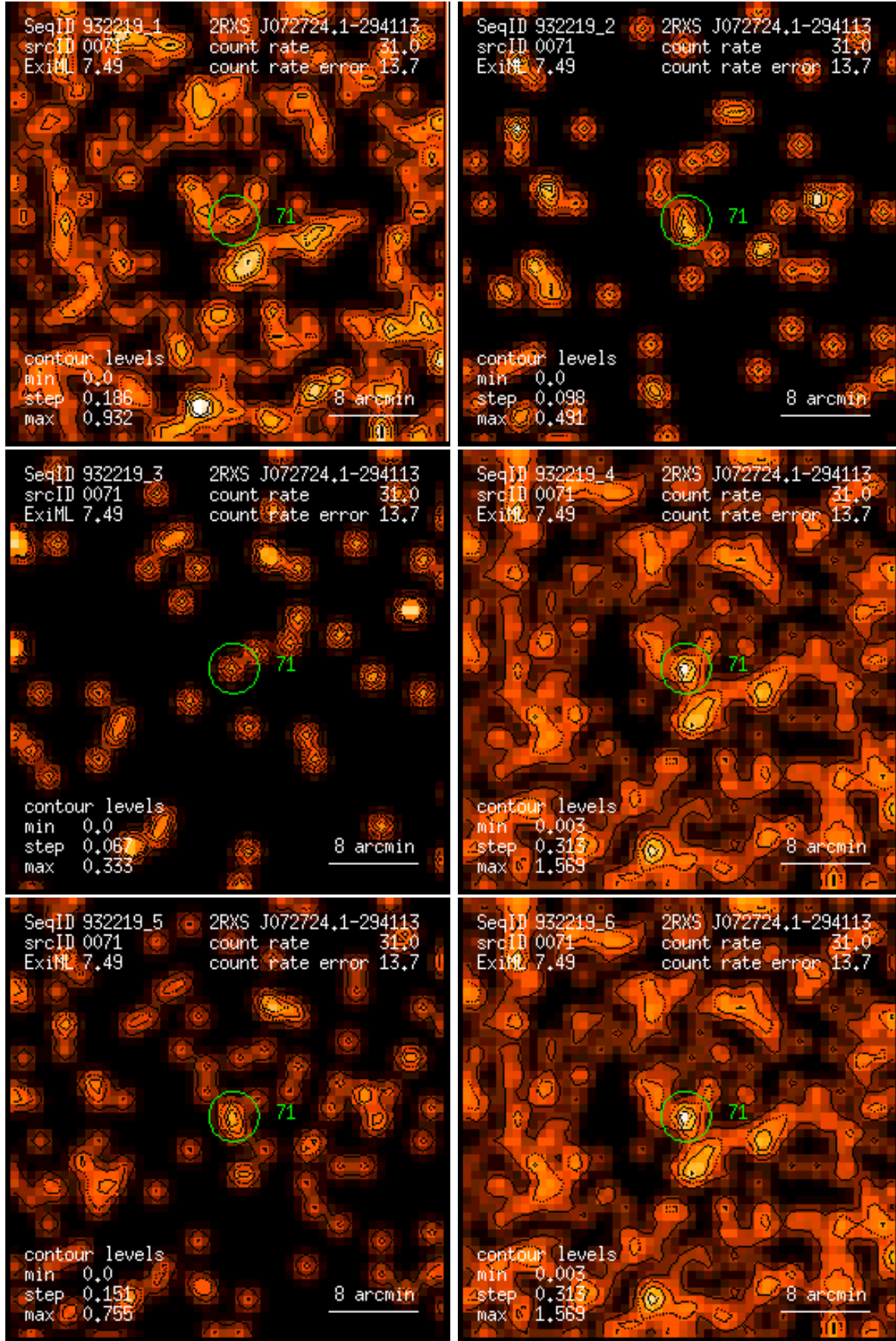
Figure 71: RASS 932219: detection 0071: band rate images, Gaussian filter: (1) PSPC channels 11 – 41, (2) 52 – 90, (3) 91 – 201, (4) 11 – 235, (5) 52 – 201, (6) 11 – 201. Broad band rates in counts/ks. Band rate contour levels in counts/ks/arcmin 2 .
