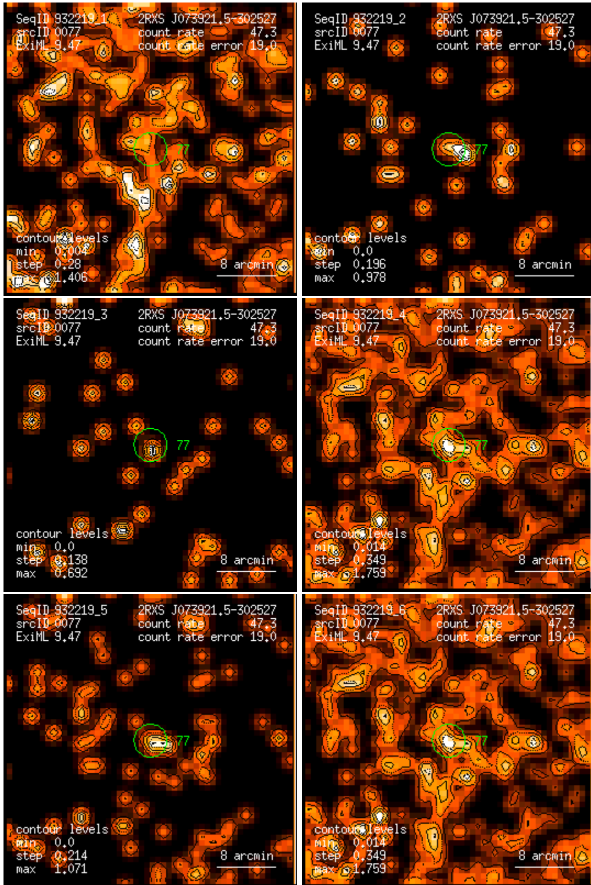
Figure 77: RASS 932219: detection 0077: band rate images, Gaussian filter: (1) PSPC channels 11 – 41, (2) 52 – 90, (3) 91 – 201, (4) 11 – 235, (5) 52 – 201, (6) 11 – 201. Broad band rates in counts/ks. Band rate contour levels in counts/ks/arcmin 2 .
