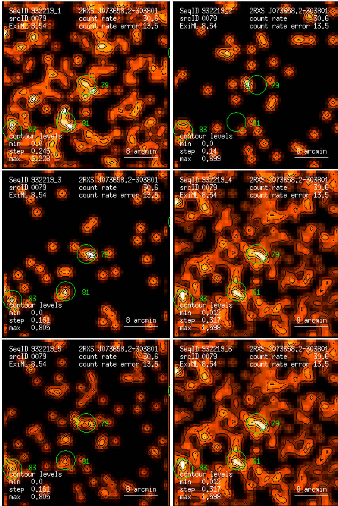
Figure 79: RASS 932219: detection 0079: band rate images, Gaussian filter: (1) PSPC channels 11 – 41, (2) 52 – 90, (3) 91 – 201, (4) 11 – 235, (5) 52 – 201, (6) 11 – 201. Broad band rates in counts/ks. Band rate contour levels in counts/ks/arcmin 2 .
