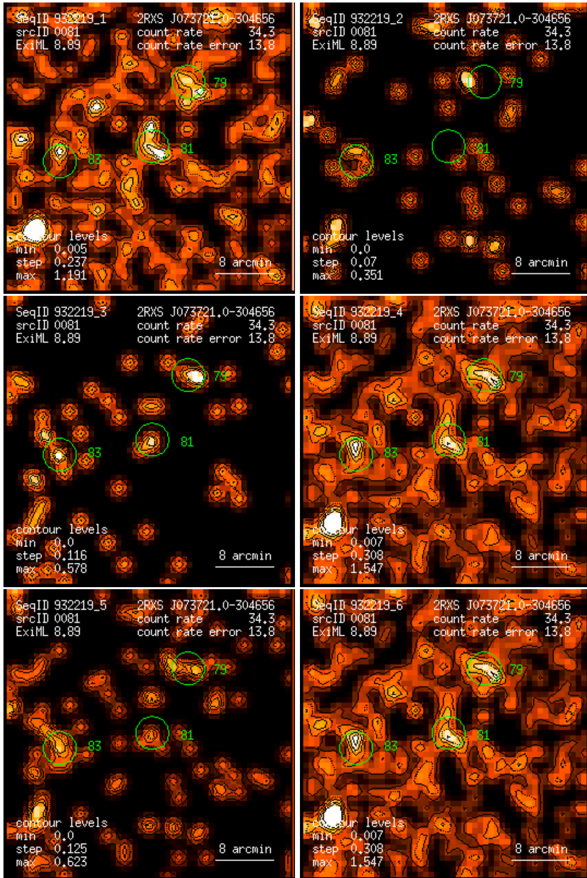
Figure 81: RASS 932219: detection 0081: band rate images, Gaussian filter: (1) PSPC channels 11 – 41, (2) 52 – 90, (3) 91 – 201, (4) 11 – 235, (5) 52 – 201, (6) 11 – 201. Broad band rates in counts/ks. Band rate contour levels in counts/ks/arcmin 2 .
