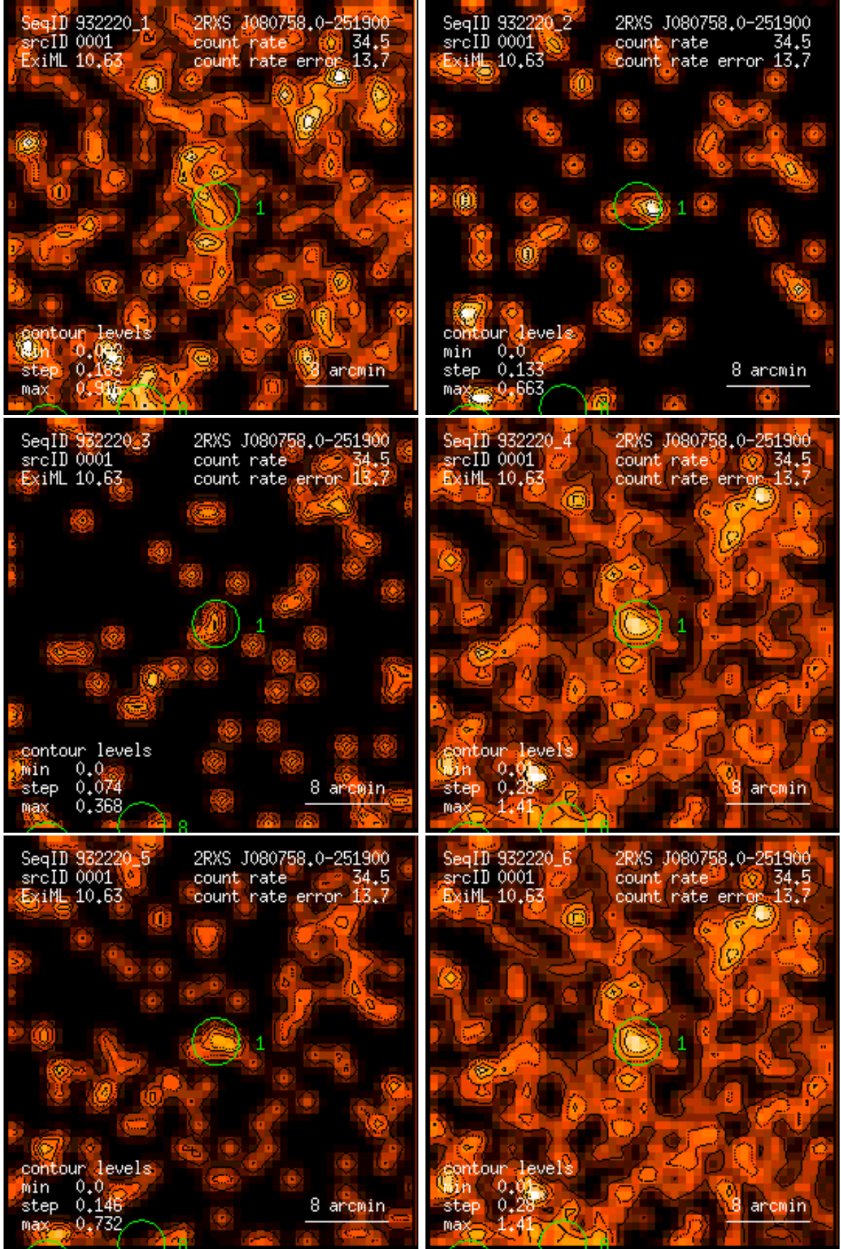
Figure 1: RASS 932220: detection 0001: band rate images, Gaussian filter: (1) PSPC channels 11 – 41, (2) 52 – 90, (3) 91 – 201, (4) 11 – 235, (5) 52 – 201, (6) 11 – 201. Broad band rates in counts/ks. Band rate contour levels in counts/ks/arcmin 2 .
