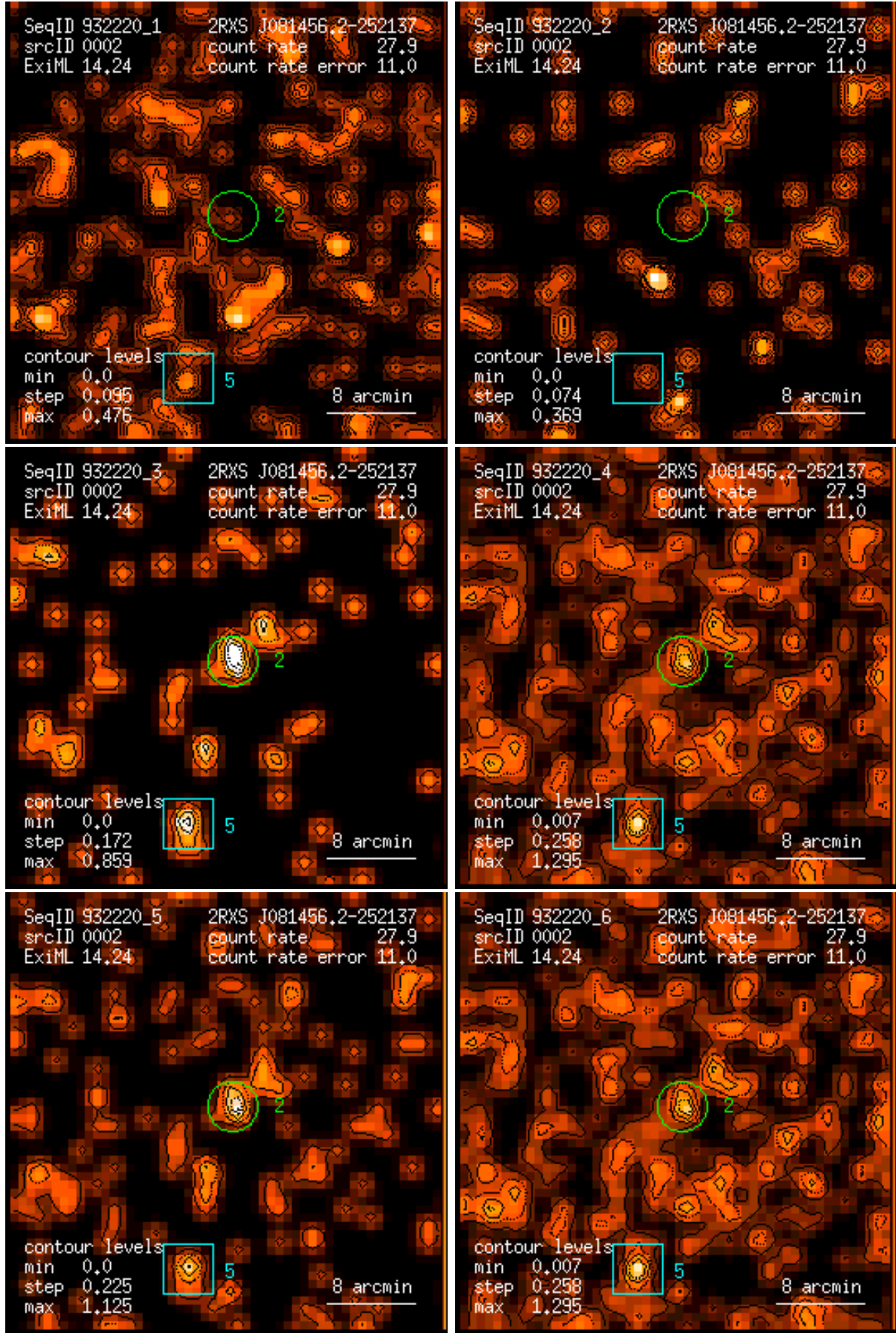
Figure 2: RASS 932220: detection 0002: band rate images, Gaussian filter: (1) PSPC channels 11 – 41, (2) 52 – 90, (3) 91 – 201, (4) 11 – 235, (5) 52 – 201, (6) 11 – 201. Broad band rates in counts/ks. Band rate contour levels in counts/ks/arcmin 2 .
