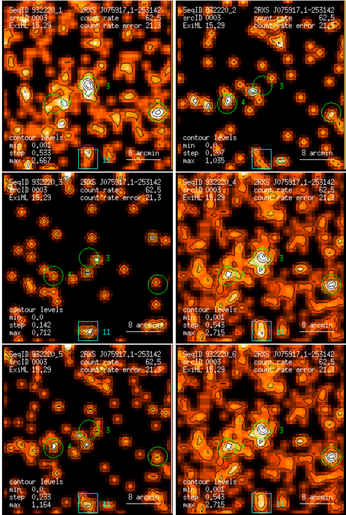
Figure 3: RASS 932220: detection 0003: band rate images, Gaussian filter: (1) PSPC channels 11 – 41, (2) 52 – 90, (3) 91 – 201, (4) 11 – 235, (5) 52 – 201, (6) 11 – 201. Broad band rates in counts/ks. Band rate contour levels in counts/ks/arcmin 2 .
