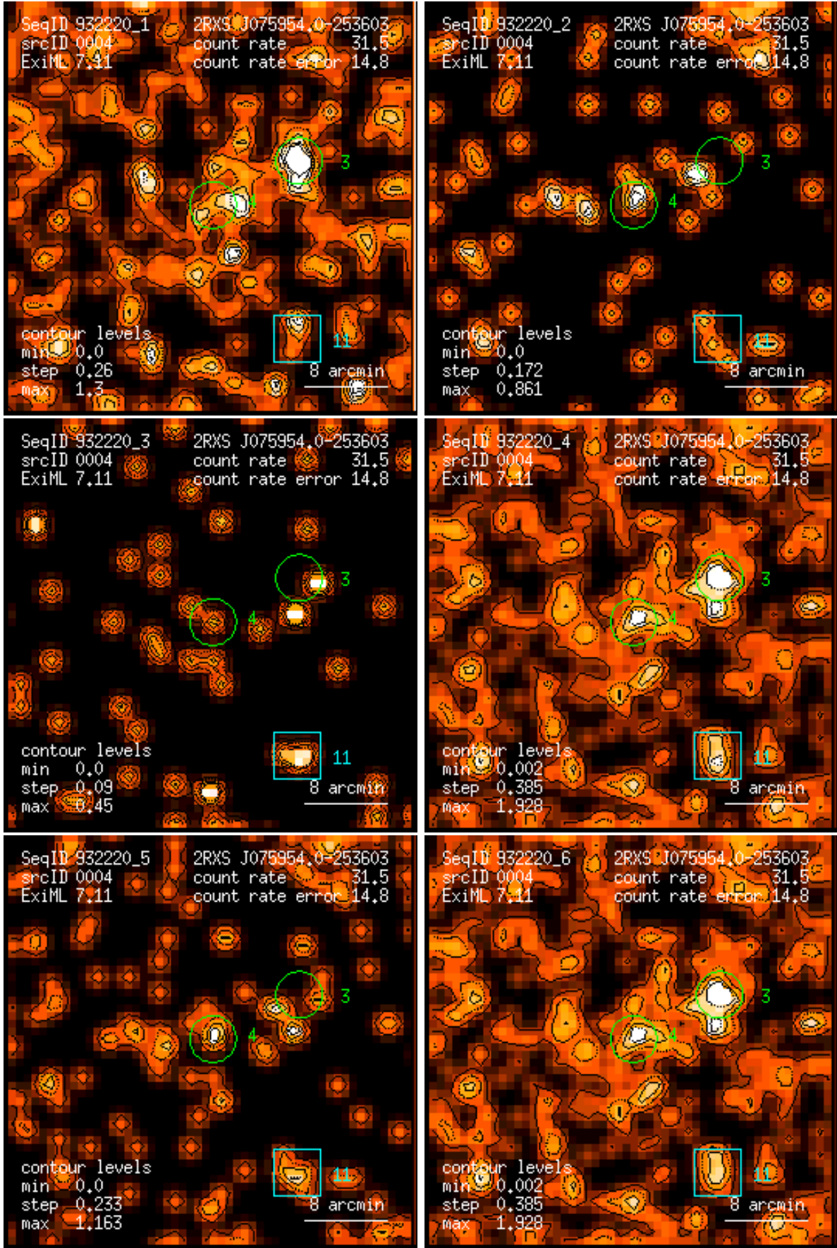
Figure 4: RASS 932220: detection 0004: band rate images, Gaussian filter: (1) PSPC channels 11 – 41, (2) 52 – 90, (3) 91 – 201, (4) 11 – 235, (5) 52 – 201, (6) 11 – 201. Broad band rates in counts/ks. Band rate contour levels in counts/ks/arcmin 2 .
