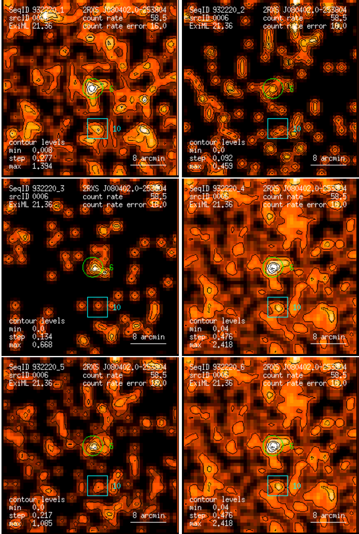
Figure 6: RASS 932220: detection 0006: band rate images, Gaussian filter: (1) PSPC channels 11 – 41, (2) 52 – 90, (3) 91 – 201, (4) 11 – 235, (5) 52 – 201, (6) 11 – 201. Broad band rates in counts/ks. Band rate contour levels in counts/ks/arcmin 2 .
