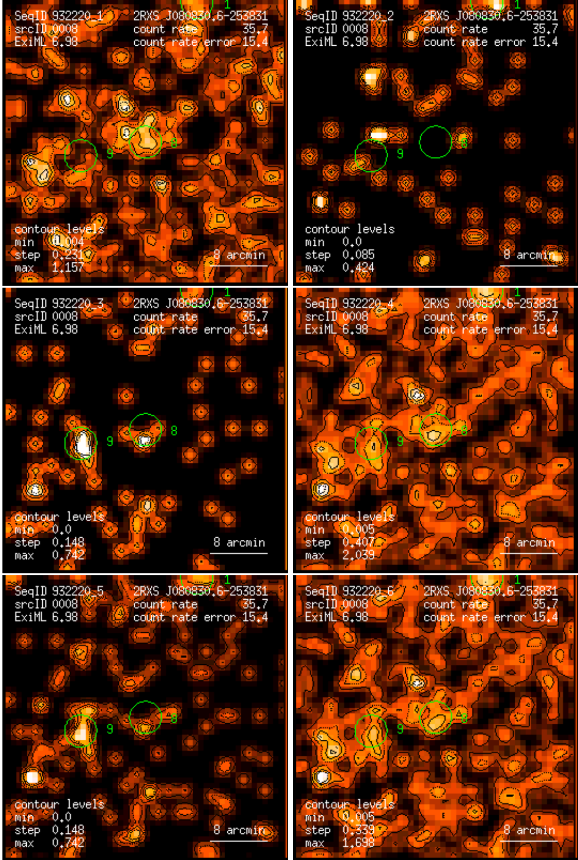
Figure 8: RASS 932220: detection 0008: band rate images, Gaussian filter: (1) PSPC channels 11 – 41, (2) 52 – 90, (3) 91 – 201, (4) 11 – 235, (5) 52 – 201, (6) 11 – 201. Broad band rates in counts/ks. Band rate contour levels in counts/ks/arcmin 2 .
