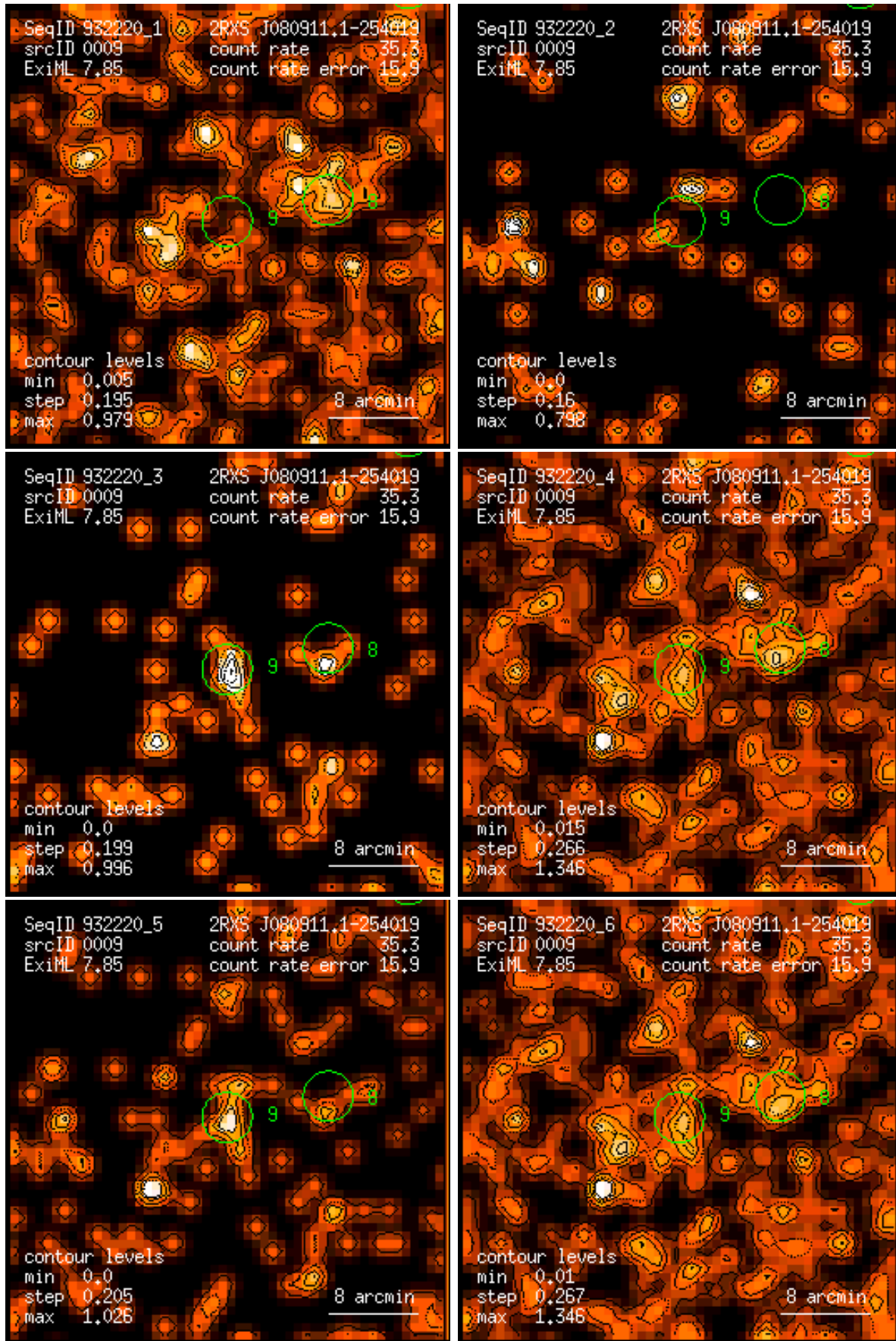
Figure 9: RASS 932220: detection 0009: band rate images, Gaussian filter: (1) PSPC channels 11 – 41, (2) 52 – 90, (3) 91 – 201, (4) 11 – 235, (5) 52 – 201, (6) 11 – 201. Broad band rates in counts/ks. Band rate contour levels in counts/ks/arcmin 2 .
