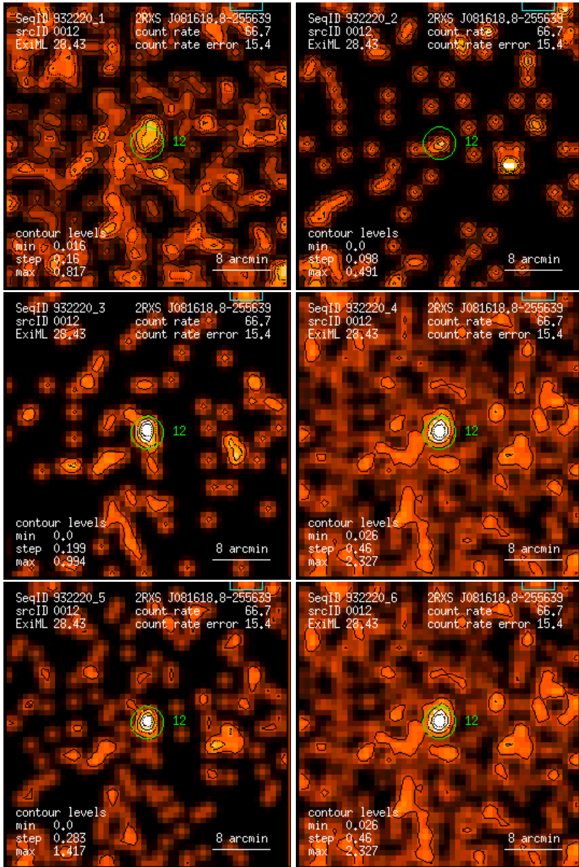
Figure 12: RASS 932220: detection 0012: band rate images, Gaussian filter: (1) PSPC channels 11 – 41, (2) 52 – 90, (3) 91 – 201, (4) 11 – 235, (5) 52 – 201, (6) 11 – 201. Broad band rates in counts/ks. Band rate contour levels in counts/ks/arcmin 2 .
