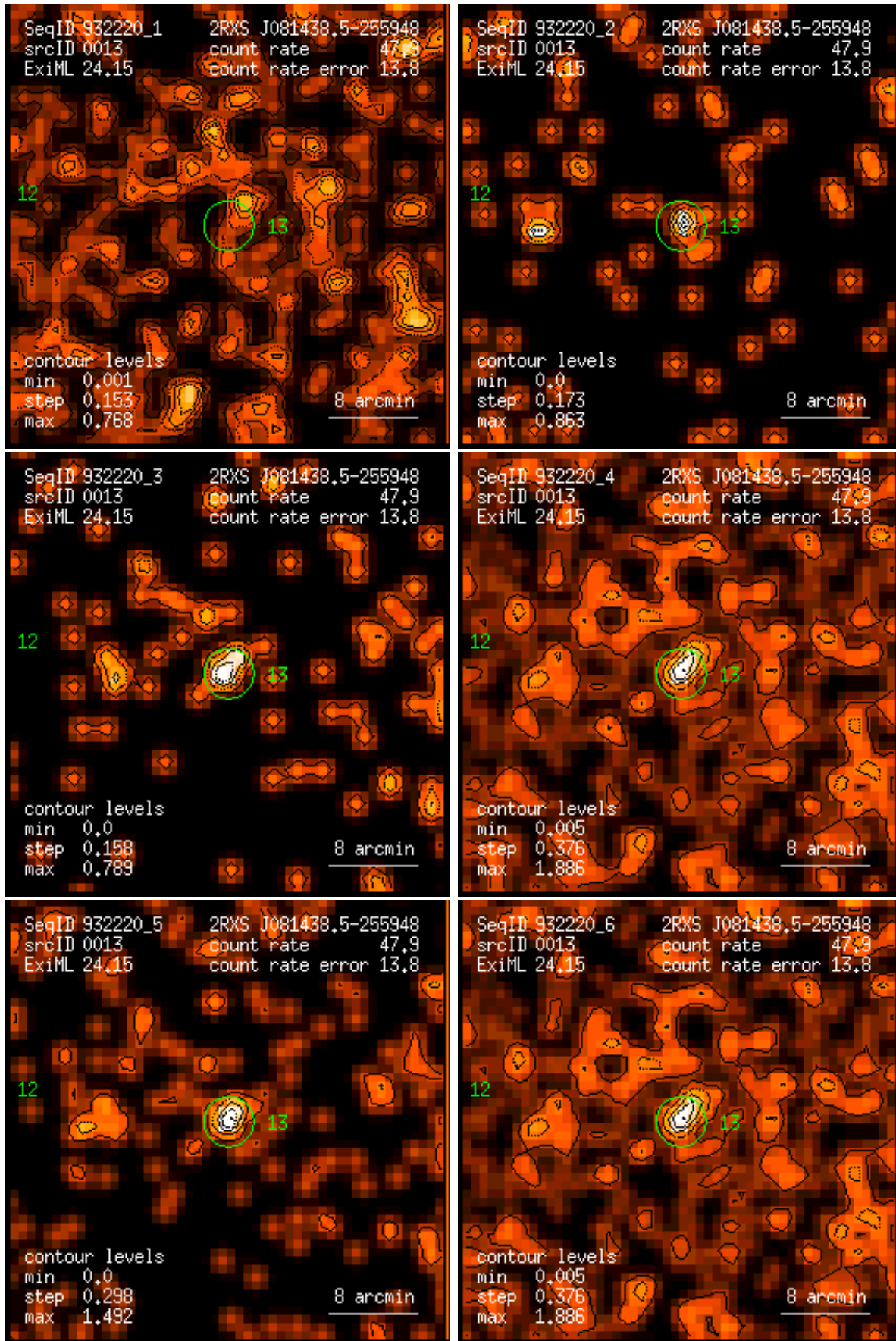
Figure 13: RASS 932220: detection 0013: band rate images, Gaussian filter: (1) PSPC channels 11 – 41, (2) 52 – 90, (3) 91 – 201, (4) 11 – 235, (5) 52 – 201, (6) 11 – 201. Broad band rates in counts/ks. Band rate contour levels in counts/ks/arcmin 2 .
