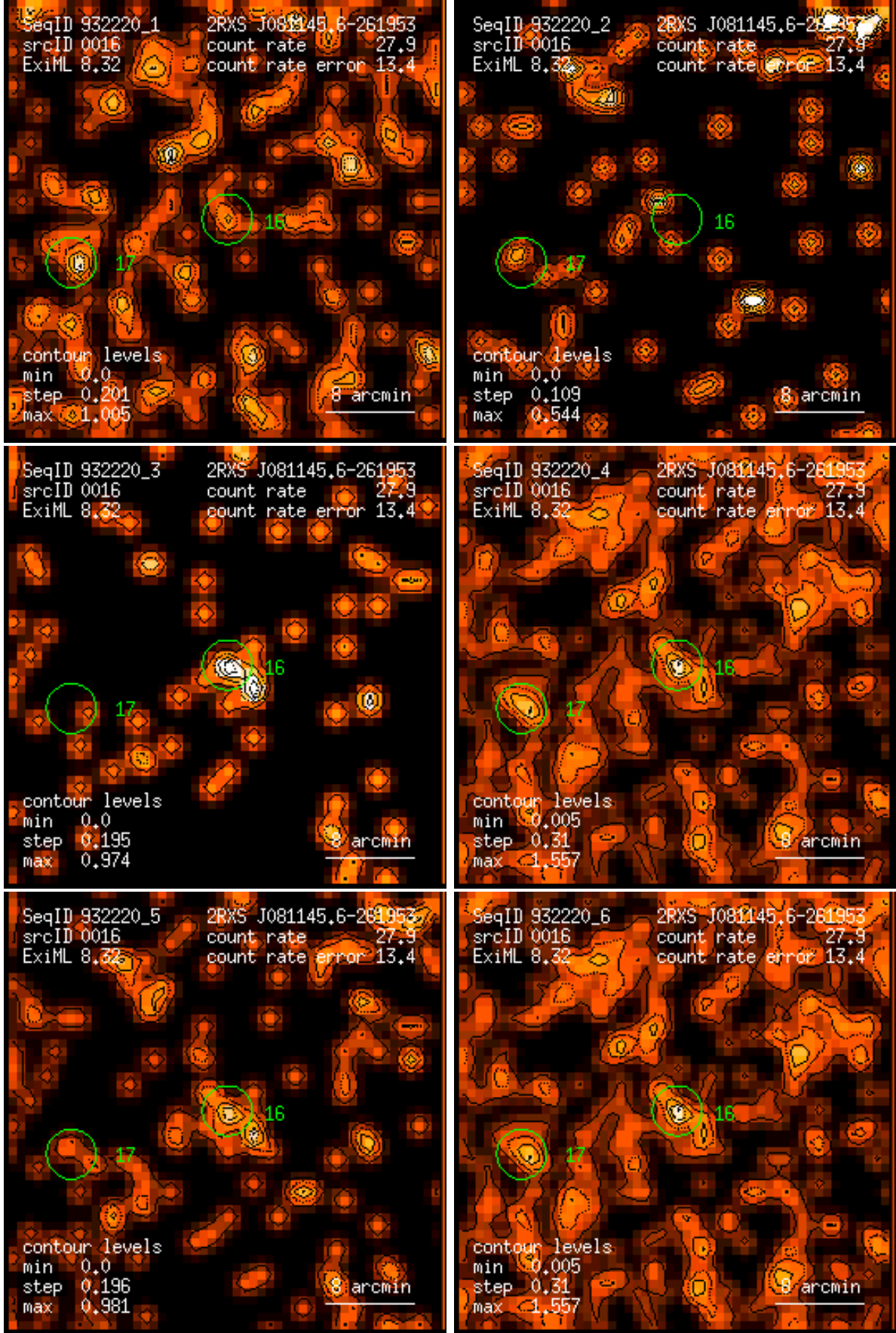
Figure 16: RASS 932220: detection 0016: band rate images, Gaussian filter: (1) PSPC channels 11 – 41, (2) 52 – 90, (3) 91 – 201, (4) 11 – 235, (5) 52 – 201, (6) 11 – 201. Broad band rates in counts/ks. Band rate contour levels in counts/ks/arcmin 2 .
