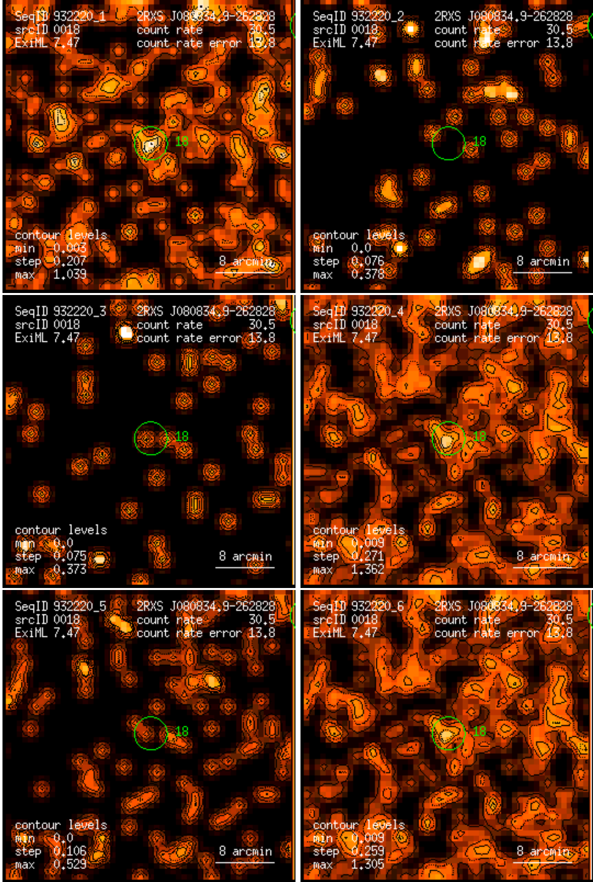
Figure 18: RASS 932220: detection 0018: band rate images, Gaussian filter: (1) PSPC channels 11 – 41, (2) 52 – 90, (3) 91 – 201, (4) 11 – 235, (5) 52 – 201, (6) 11 – 201. Broad band rates in counts/ks. Band rate contour levels in counts/ks/arcmin 2 .
