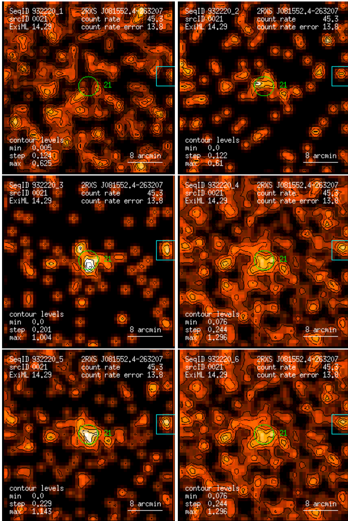
Figure 21: RASS 932220: detection 0021: band rate images, Gaussian filter: (1) PSPC channels 11 – 41, (2) 52 – 90, (3) 91 – 201, (4) 11 – 235, (5) 52 – 201, (6) 11 – 201. Broad band rates in counts/ks. Band rate contour levels in counts/ks/arcmin 2 .
