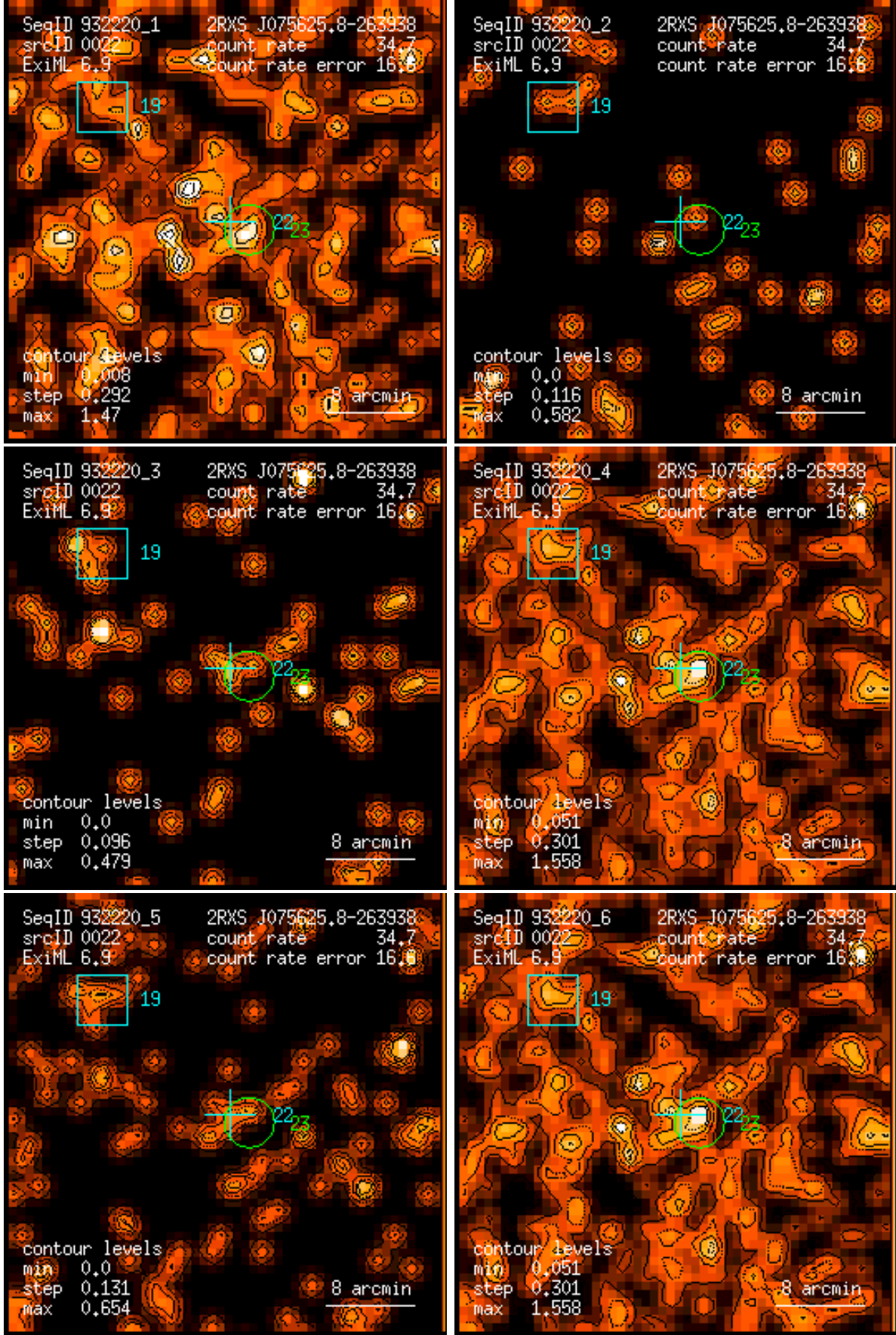
Figure 22: RASS 932220: detection 0022: band rate images, Gaussian filter: (1) PSPC channels 11 – 41, (2) 52 – 90, (3) 91 – 201, (4) 11 – 235, (5) 52 – 201, (6) 11 – 201. Broad band rates in counts/ks. Band rate contour levels in counts/ks/arcmin 2 .
