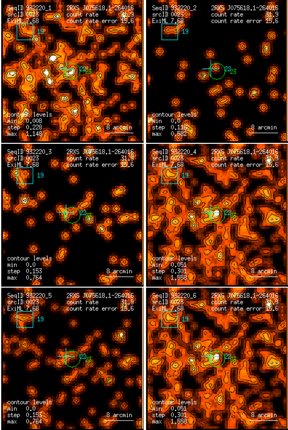
Figure 23: RASS 932220: detection 0023: band rate images, Gaussian filter: (1) PSPC channels 11 – 41, (2) 52 – 90, (3) 91 – 201, (4) 11 – 235, (5) 52 – 201, (6) 11 – 201. Broad band rates in counts/ks. Band rate contour levels in counts/ks/arcmin 2 .
