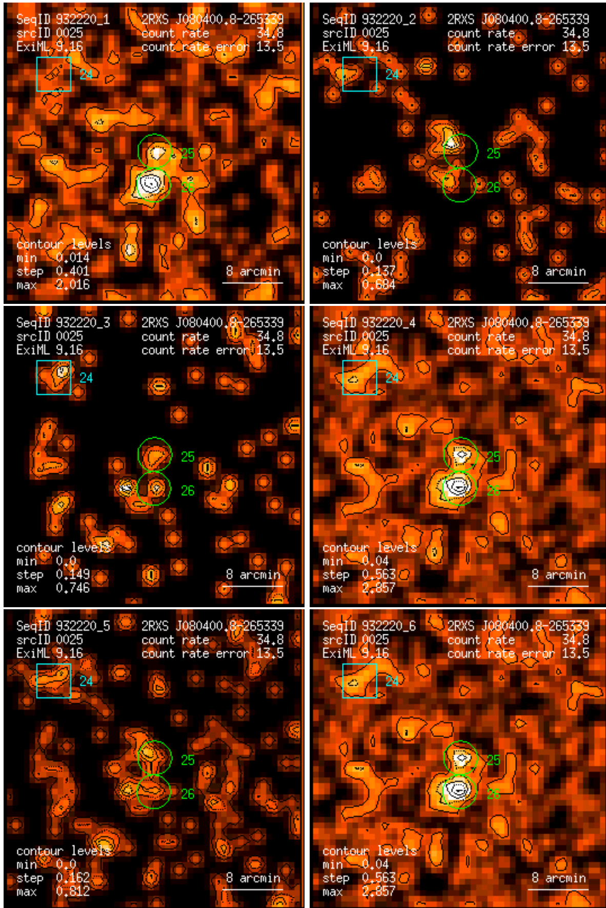
Figure 25: RASS 932220: detection 0025: band rate images, Gaussian filter: (1) PSPC channels 11 – 41, (2) 52 – 90, (3) 91 – 201, (4) 11 – 235, (5) 52 – 201, (6) 11 – 201. Broad band rates in counts/ks. Band rate contour levels in counts/ks/arcmin 2 .
