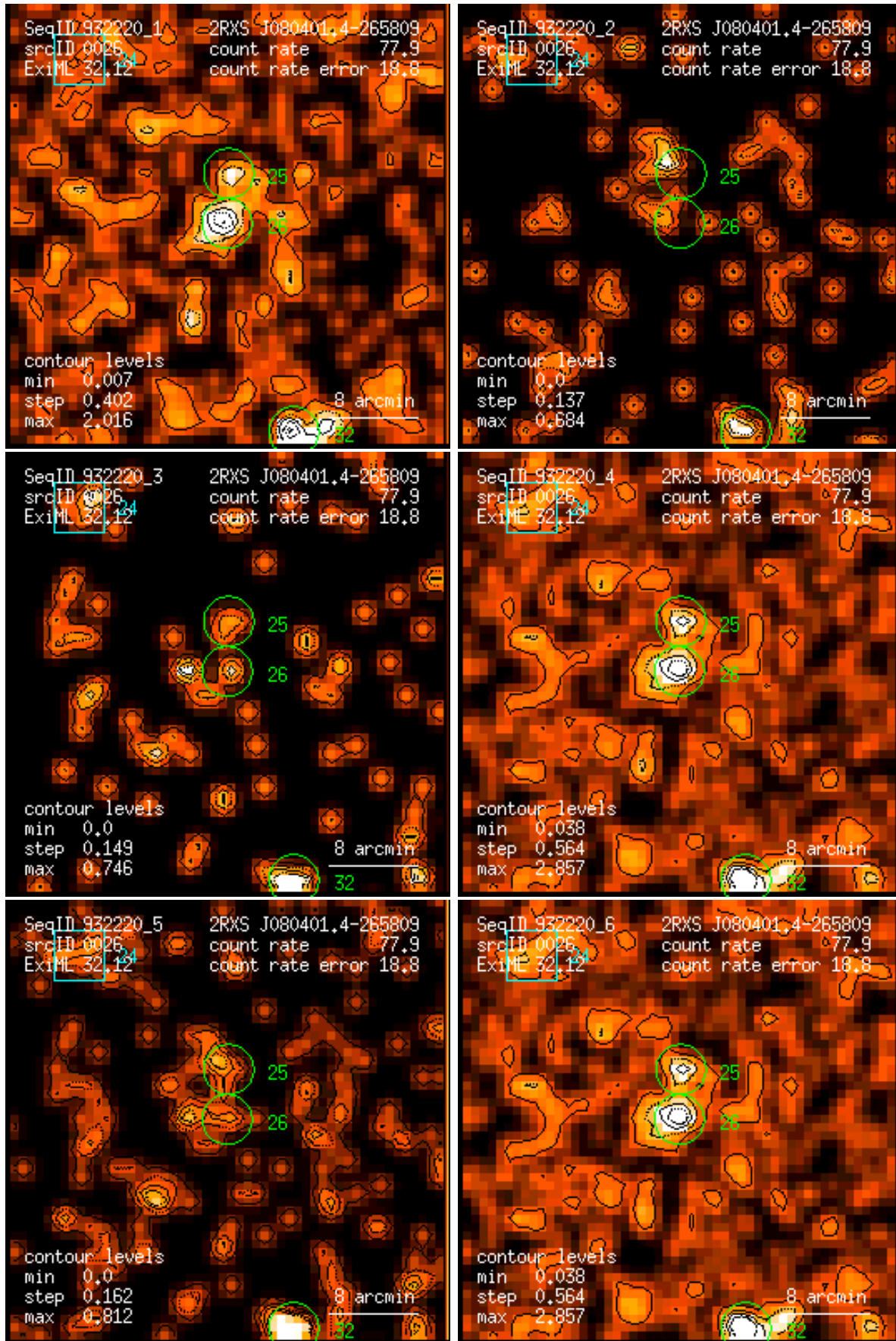
Figure 26: RASS 932220: detection 0026: band rate images, Gaussian filter: (1) PSPC channels 11 – 41, (2) 52 – 90, (3) 91 – 201, (4) 11 – 235, (5) 52 – 201, (6) 11 – 201. Broad band rates in counts/ks. Band rate contour levels in counts/ks/arcmin 2 .
