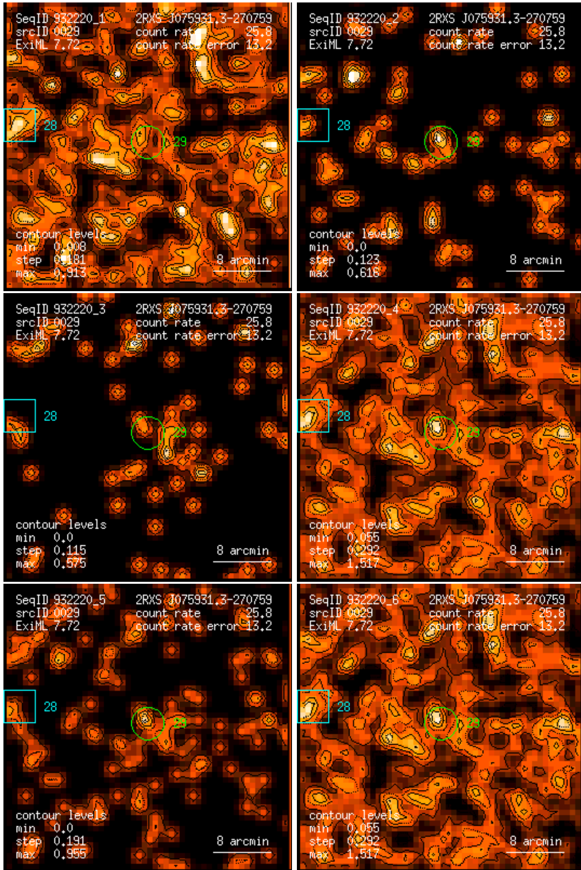
Figure 29: RASS 932220: detection 0029: band rate images, Gaussian filter: (1) PSPC channels 11 – 41, (2) 52 – 90, (3) 91 – 201, (4) 11 – 235, (5) 52 – 201, (6) 11 – 201. Broad band rates in counts/ks. Band rate contour levels in counts/ks/arcmin 2 .
