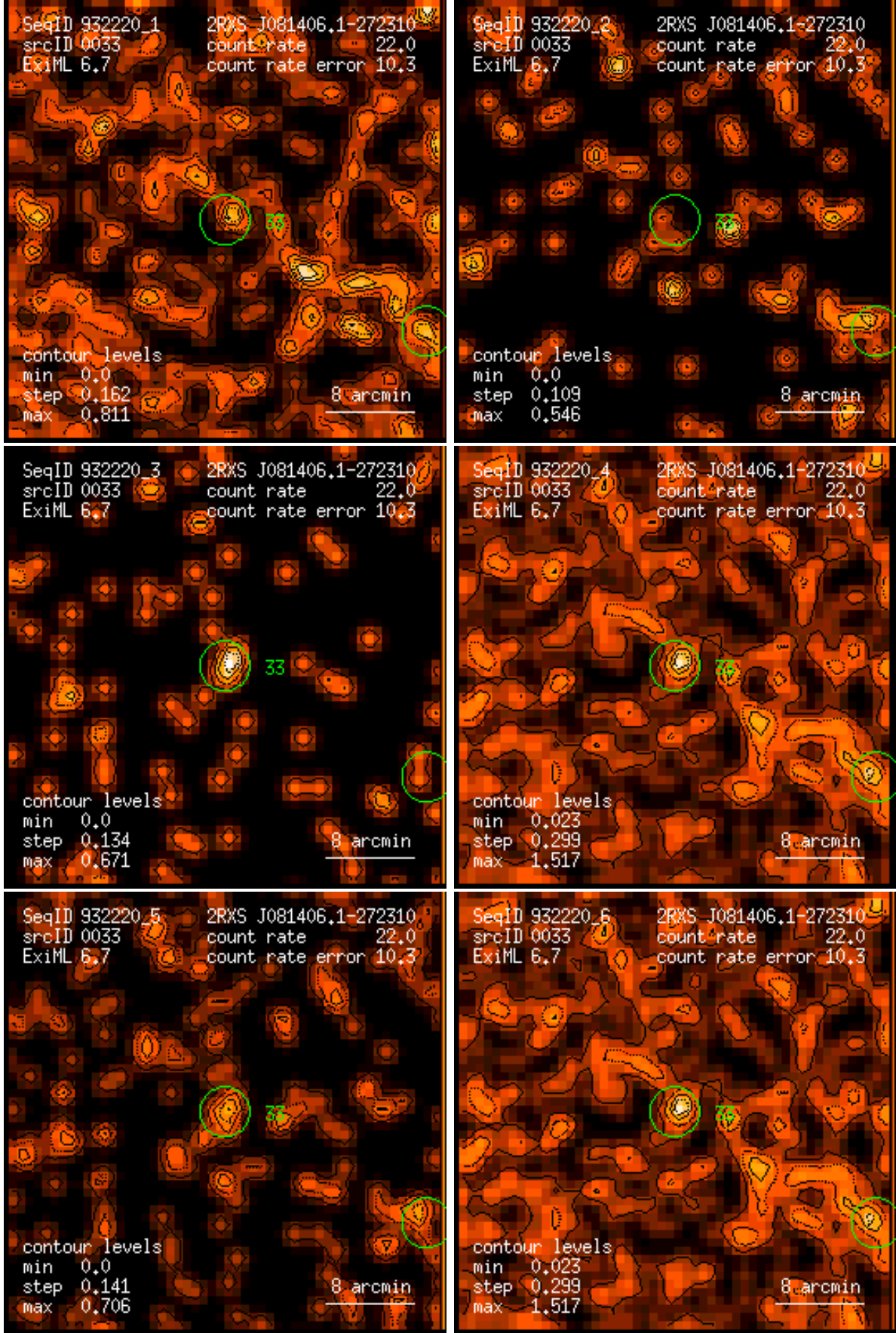
Figure 33: RASS 932220: detection 0033: band rate images, Gaussian filter: (1) PSPC channels 11 – 41, (2) 52 – 90, (3) 91 – 201, (4) 11 – 235, (5) 52 – 201, (6) 11 – 201. Broad band rates in counts/ks. Band rate contour levels in counts/ks/arcmin 2 .
