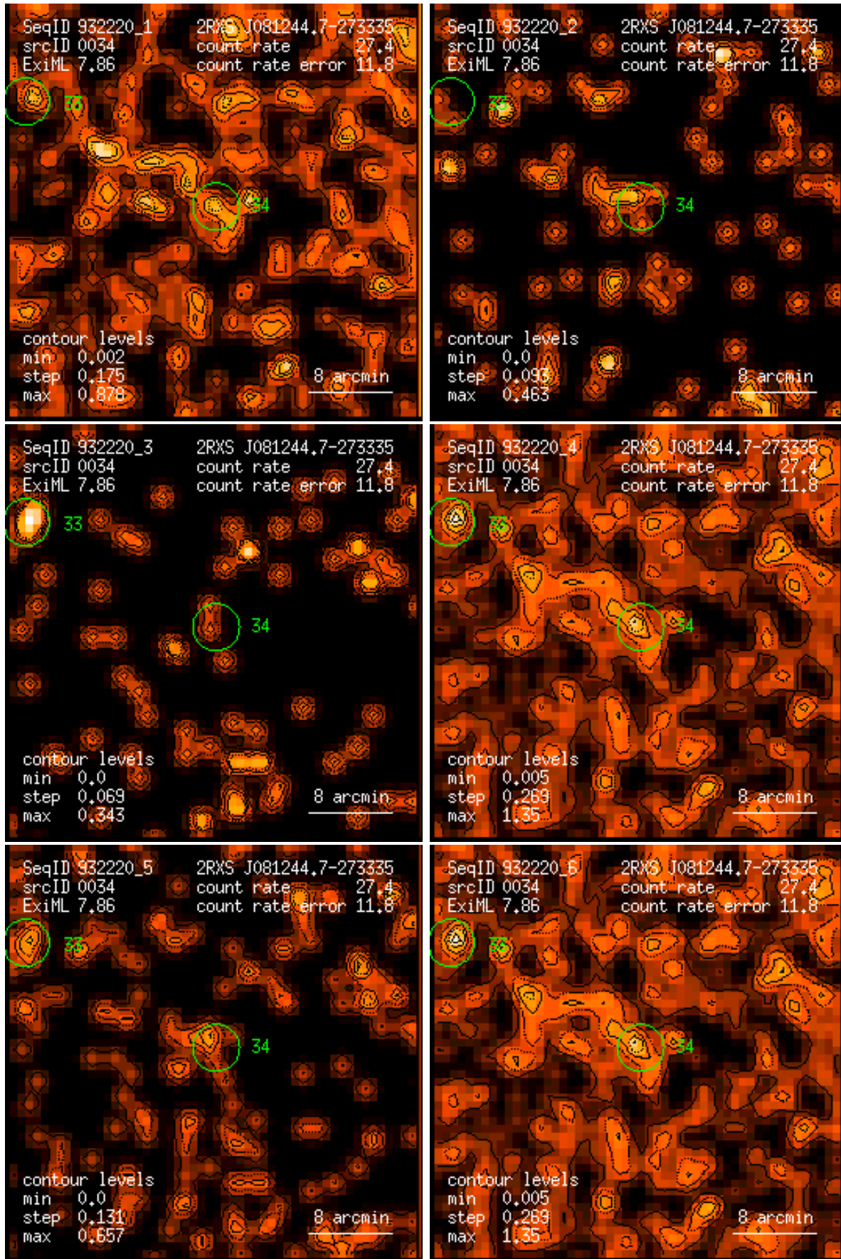
Figure 34: RASS 932220: detection 0034: band rate images, Gaussian filter: (1) PSPC channels 11 – 41, (2) 52 – 90, (3) 91 – 201, (4) 11 – 235, (5) 52 – 201, (6) 11 – 201. Broad band rates in counts/ks. Band rate contour levels in counts/ks/arcmin 2 .
