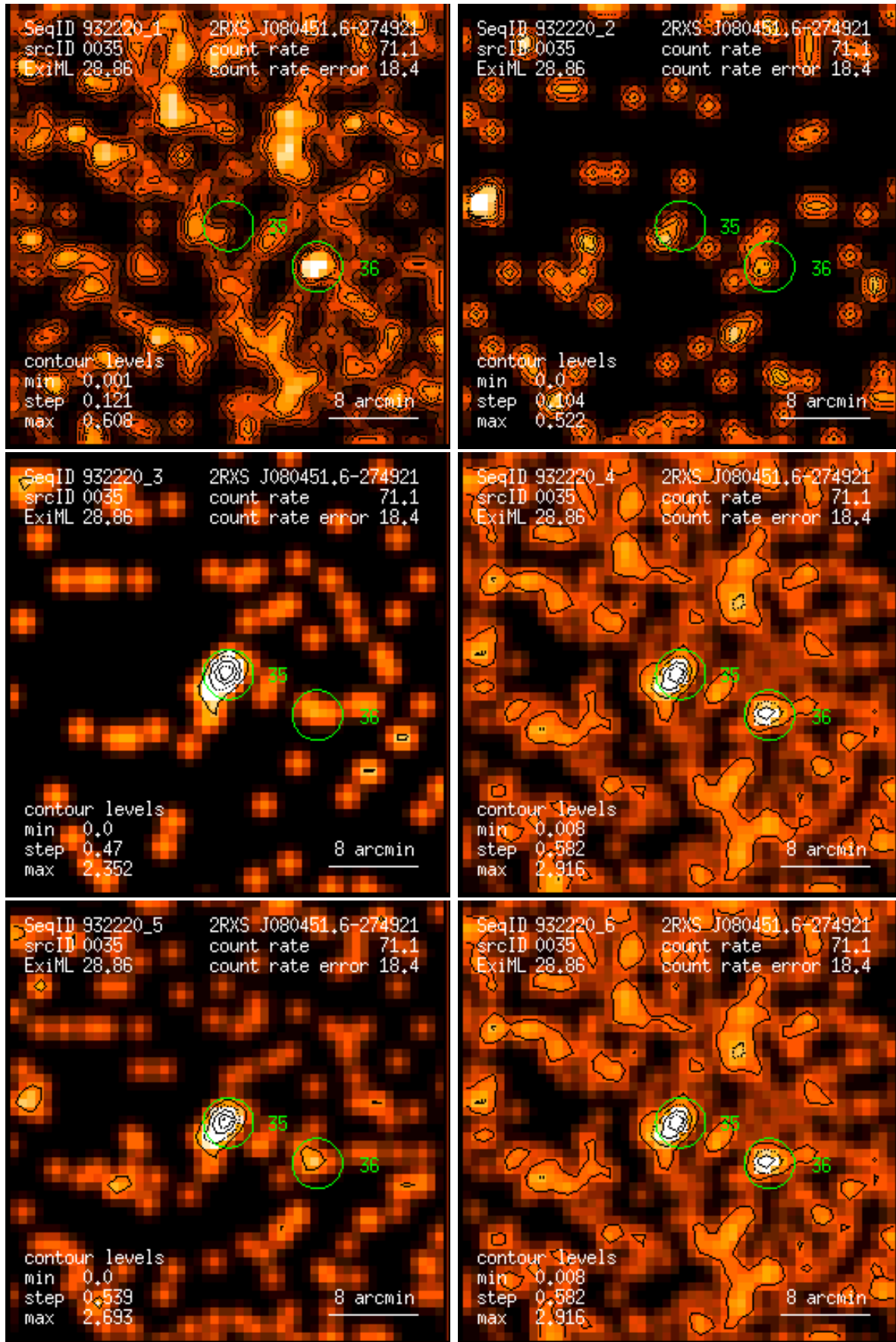
Figure 35: RASS 932220: detection 0035: band rate images, Gaussian filter: (1) PSPC channels 11 – 41, (2) 52 – 90, (3) 91 – 201, (4) 11 – 235, (5) 52 – 201, (6) 11 – 201. Broad band rates in counts/ks. Band rate contour levels in counts/ks/arcmin 2 .
