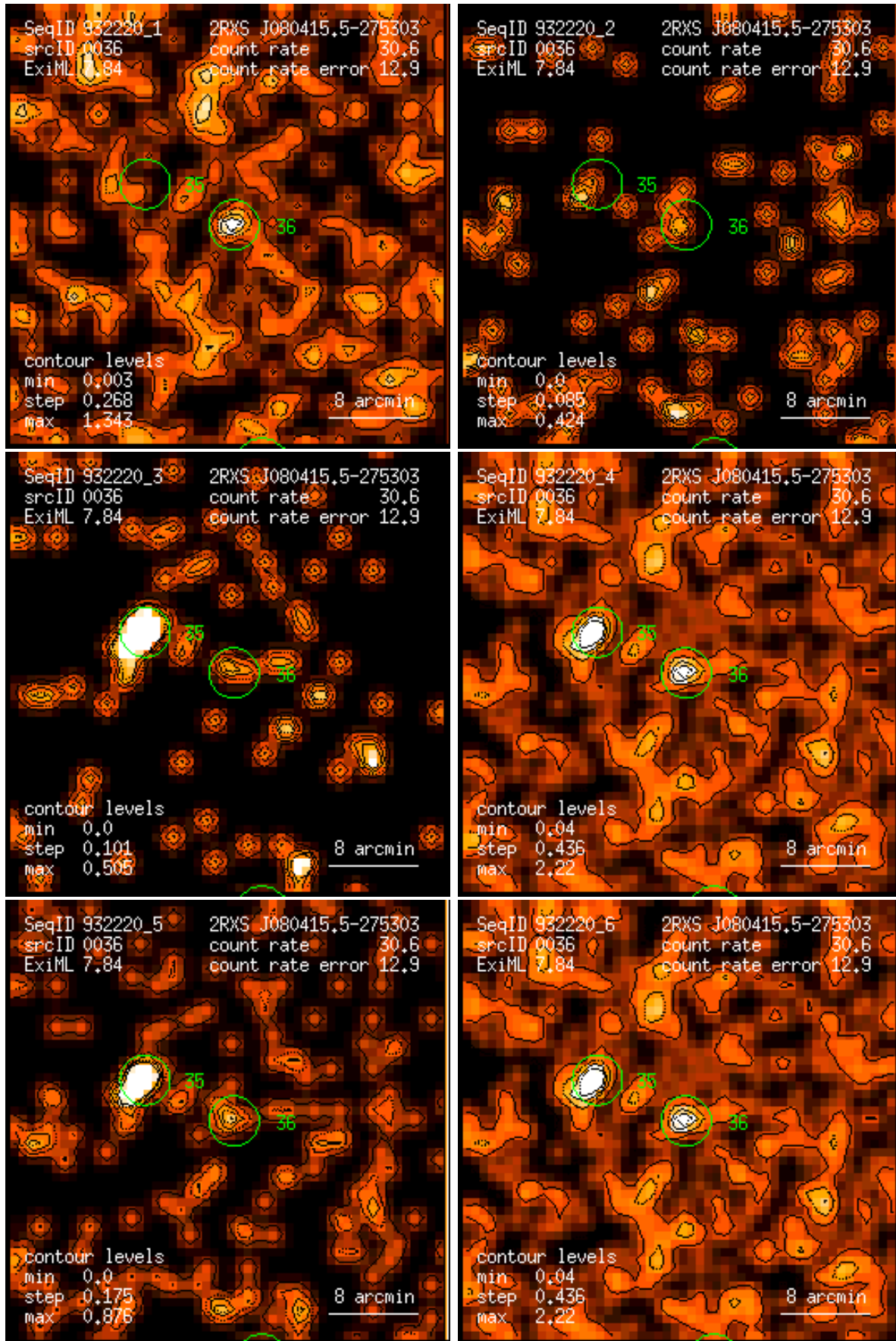
Figure 36: RASS 932220: detection 0036: band rate images, Gaussian filter: (1) PSPC channels 11 – 41, (2) 52 – 90, (3) 91 – 201, (4) 11 – 235, (5) 52 – 201, (6) 11 – 201. Broad band rates in counts/ks. Band rate contour levels in counts/ks/arcmin 2 .
